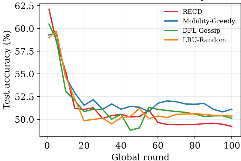
Beam-selection accuracy
