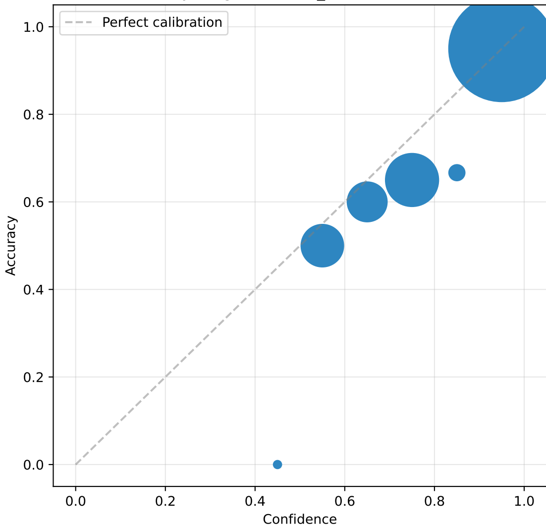
Reliability Diagram: small_world (ECE=0.0709)
