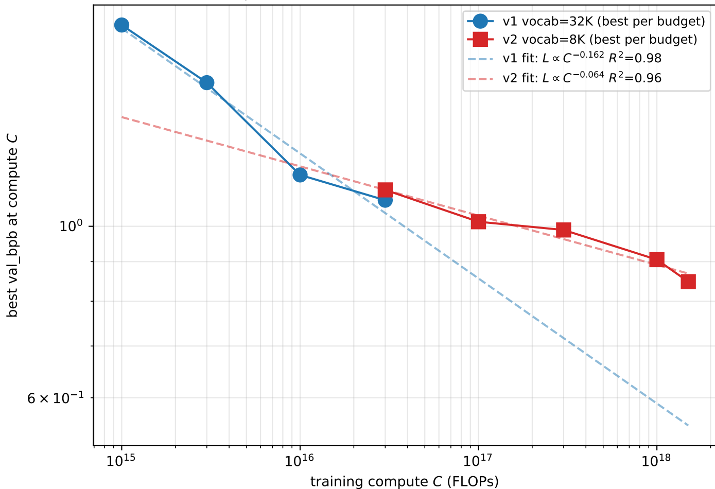
Loss vs compute — v1 (vocab=32K) vs v2 (vocab=8K) on V100
