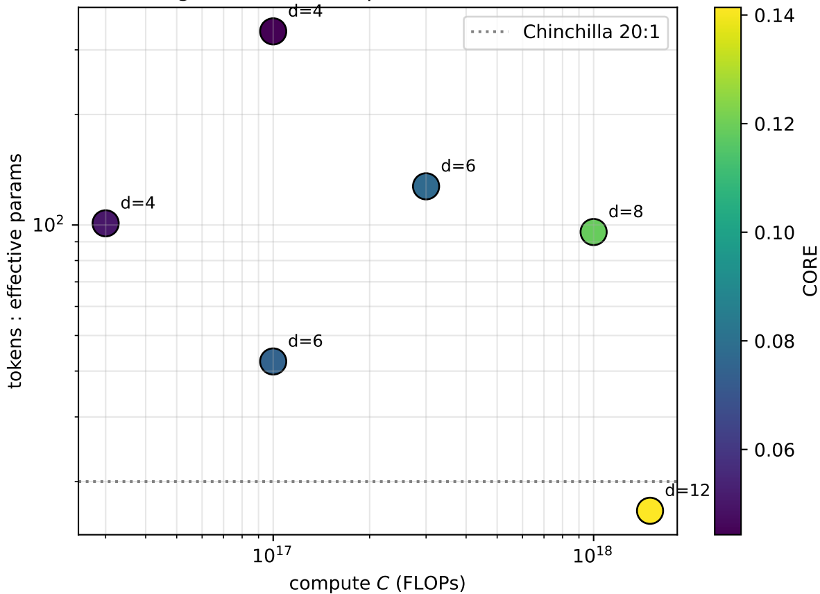
v2 emerge runs — token:param ratio (color = CORE)
