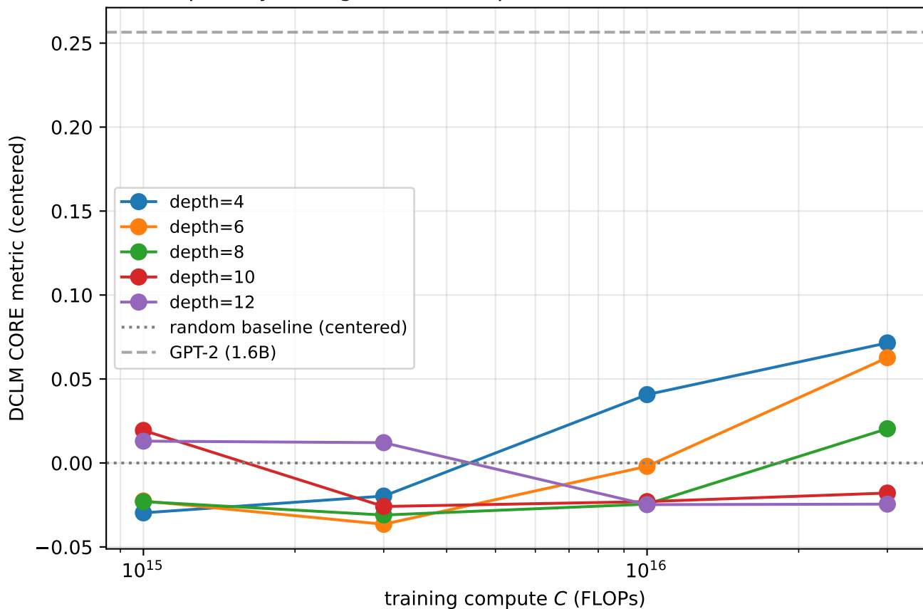
Capability emergence vs compute (V100 minimum-scale runs)
