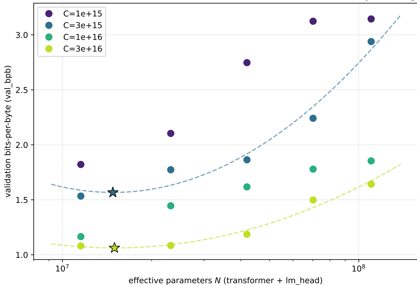
IsoFLOP curves on V100 — minimum-scale validation of Chinchilla-style scaling
