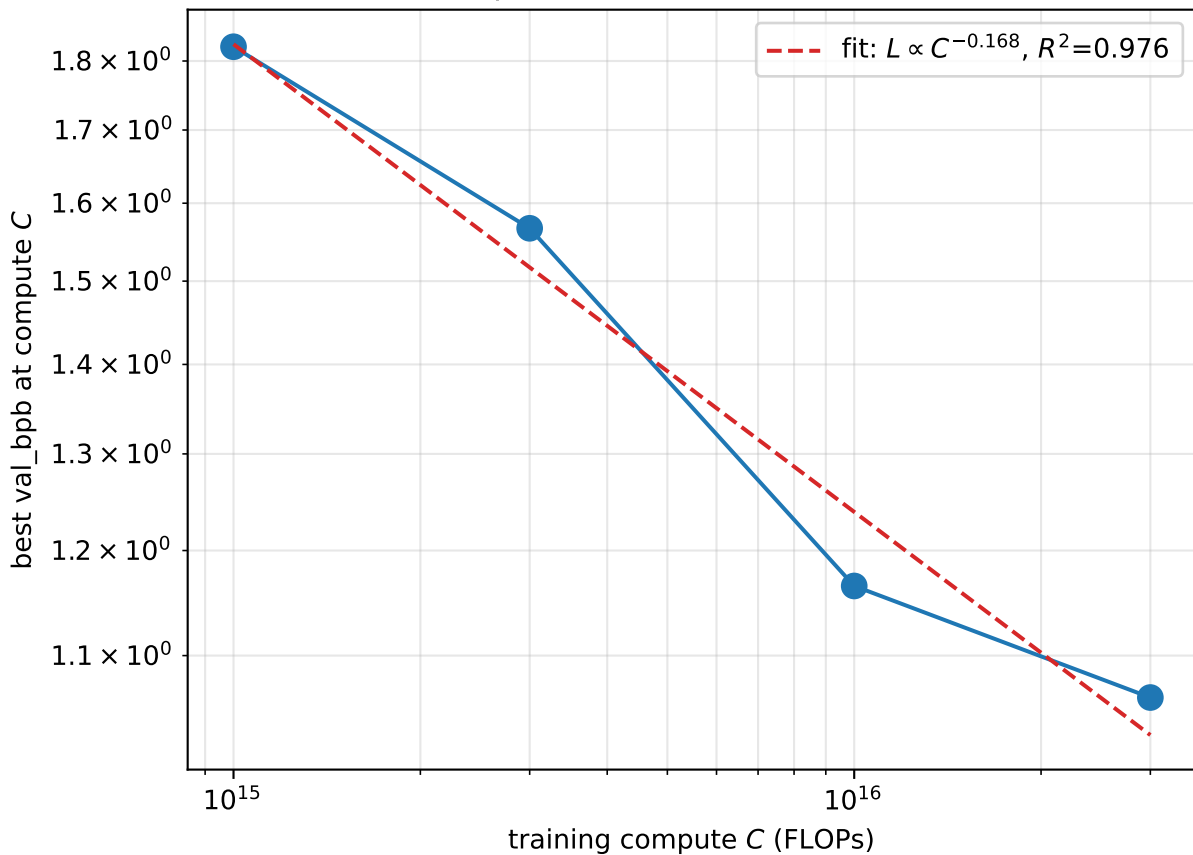
Loss vs compute — V100 minimum-scale frontier
