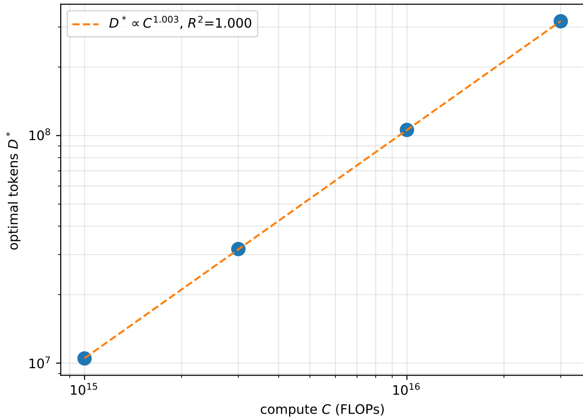
Compute-optimal data scaling
