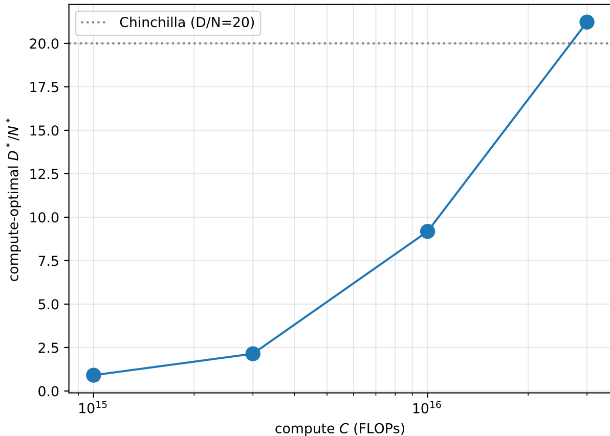
Token:param ratio along the compute-optimal frontier
