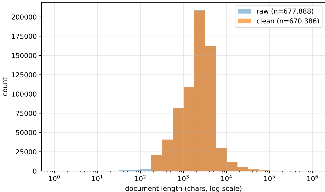
ClimbMix shard — doc length distribution, raw vs cleaned
