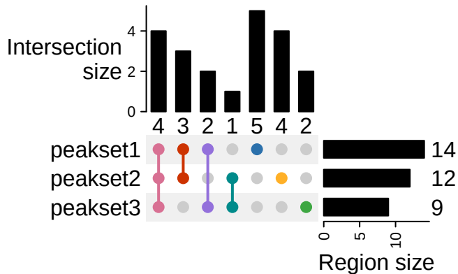
mode = "reduce"
