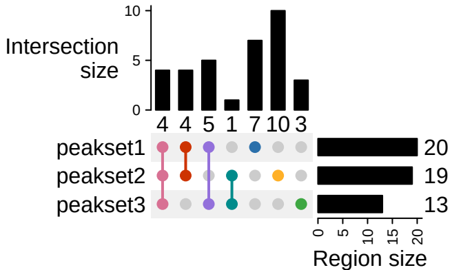
mode = "disjoin"
