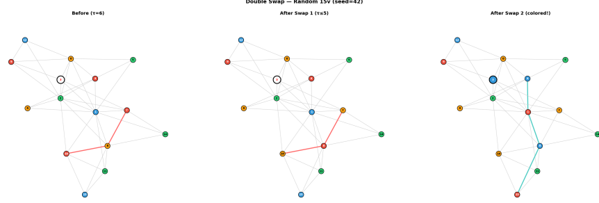
Figure 2: The double-swap mechanism on a random 15-vertex triangulation. Left: Before — vertex (white circle) is uncolored, \tau = 6 , all 6 pairs tangled. A cross-linked bridge pair is highlighted (red). Middle: After Swap 1 — split-bridge swap drops \tau to 5. Right: After Swap 2 — freed pair swapped, vertex receives its color. The Kempe chain used in Swap 2 is highlighted (cyan).
