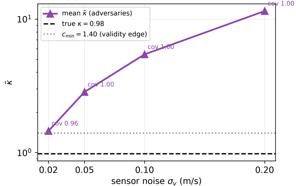
(c) Online estimate \tilde{\kappa} over-covers \kappa
