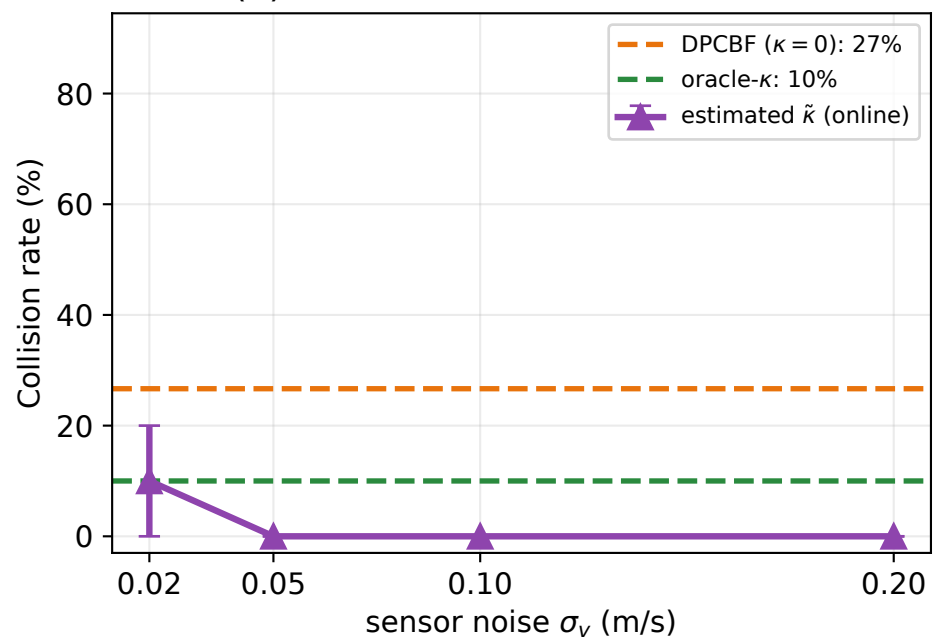
(b) Collision rate vs sensor noise
