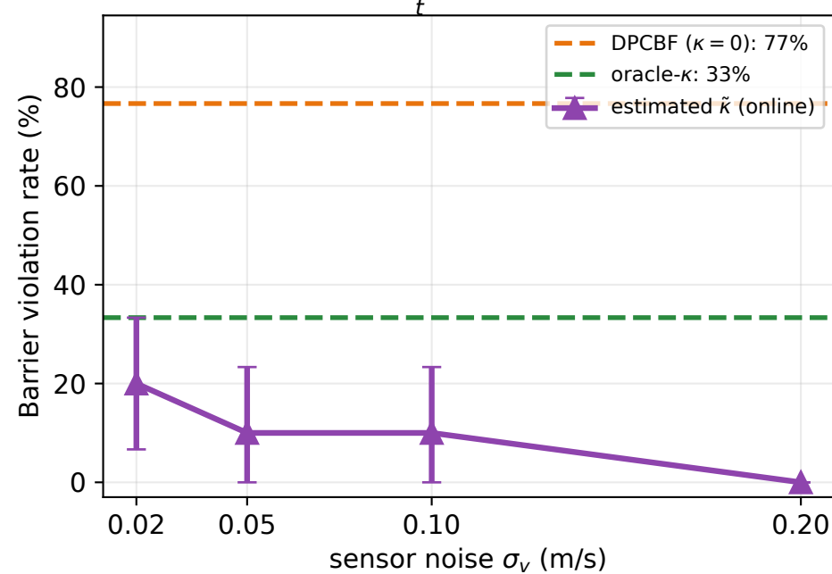
(a) Violation P[\min h < 0] vs sensor noise
