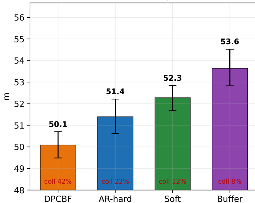
(b) Path length
