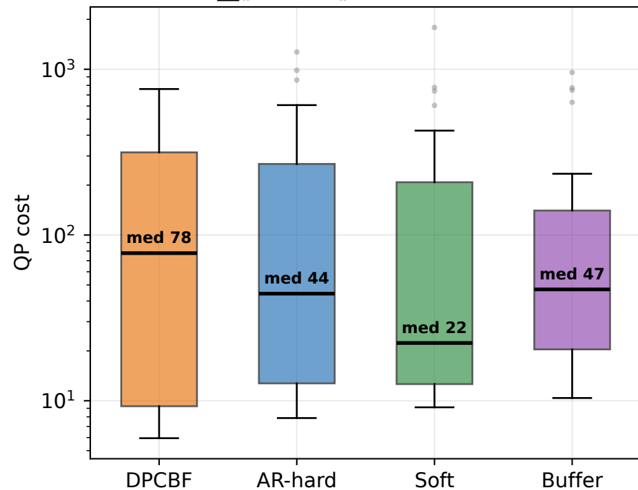
(a) QP cost \sum \|u - u_{\text{ref}}\|^2 (log, box=median/IQR)
