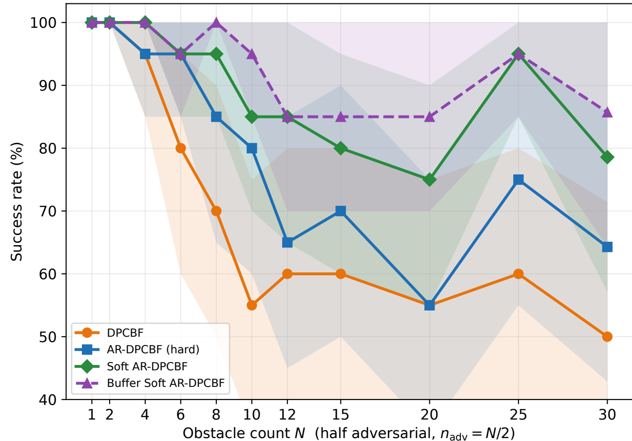
(b) Success rate vs density (reached &amp; collision-free)
