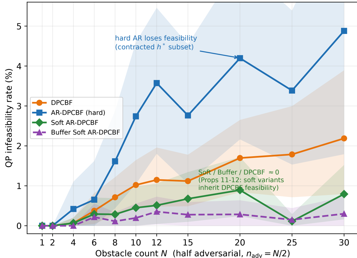
(a) QP infeasibility rate vs density
