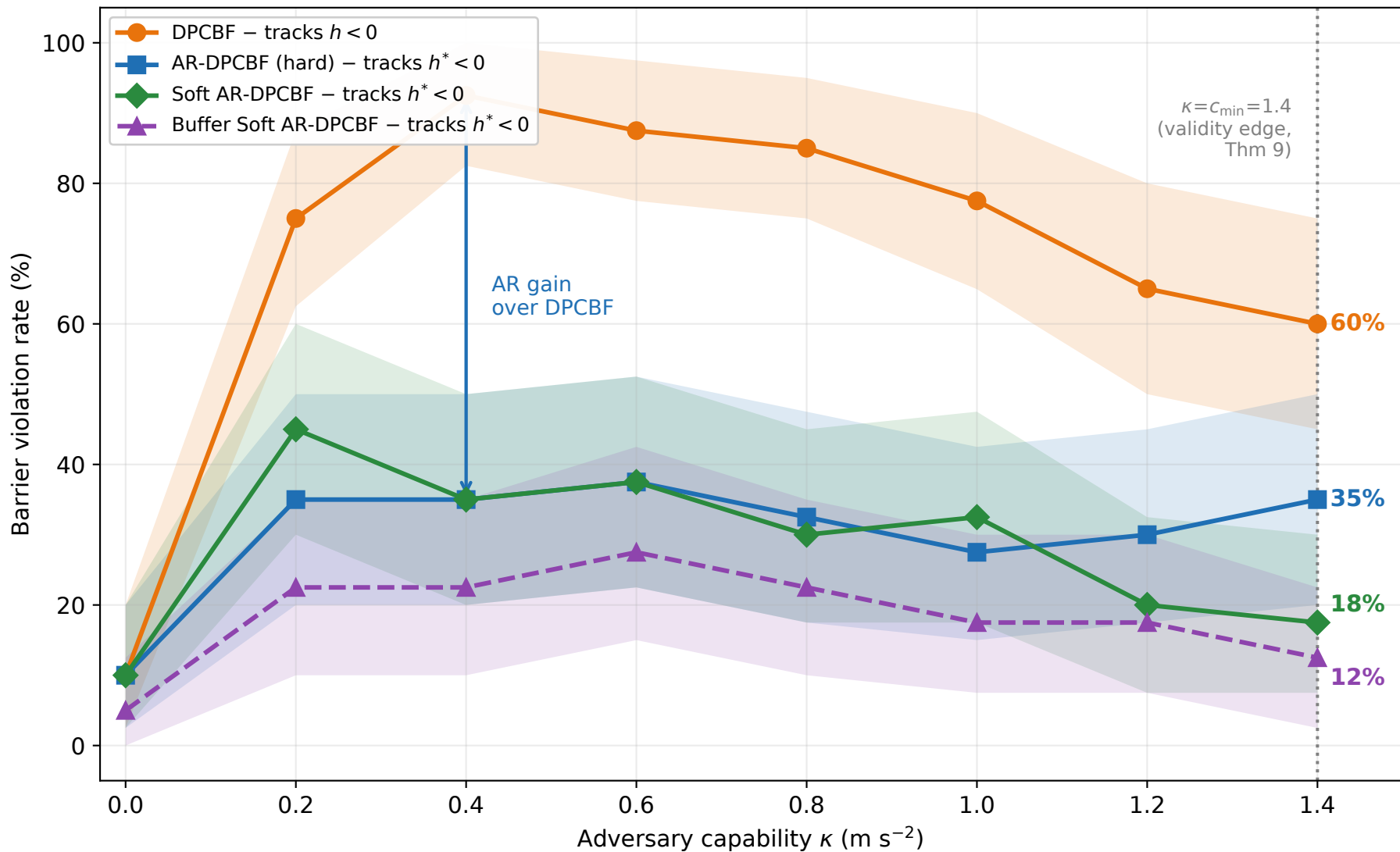
Violation rate vs adversary capability \kappa (bootstrap 95% CIs) N = 10 , n_{\text{adv}} = 5 , DPCBF Table I params, goal-reach = 100%, n = 40 trials/level
