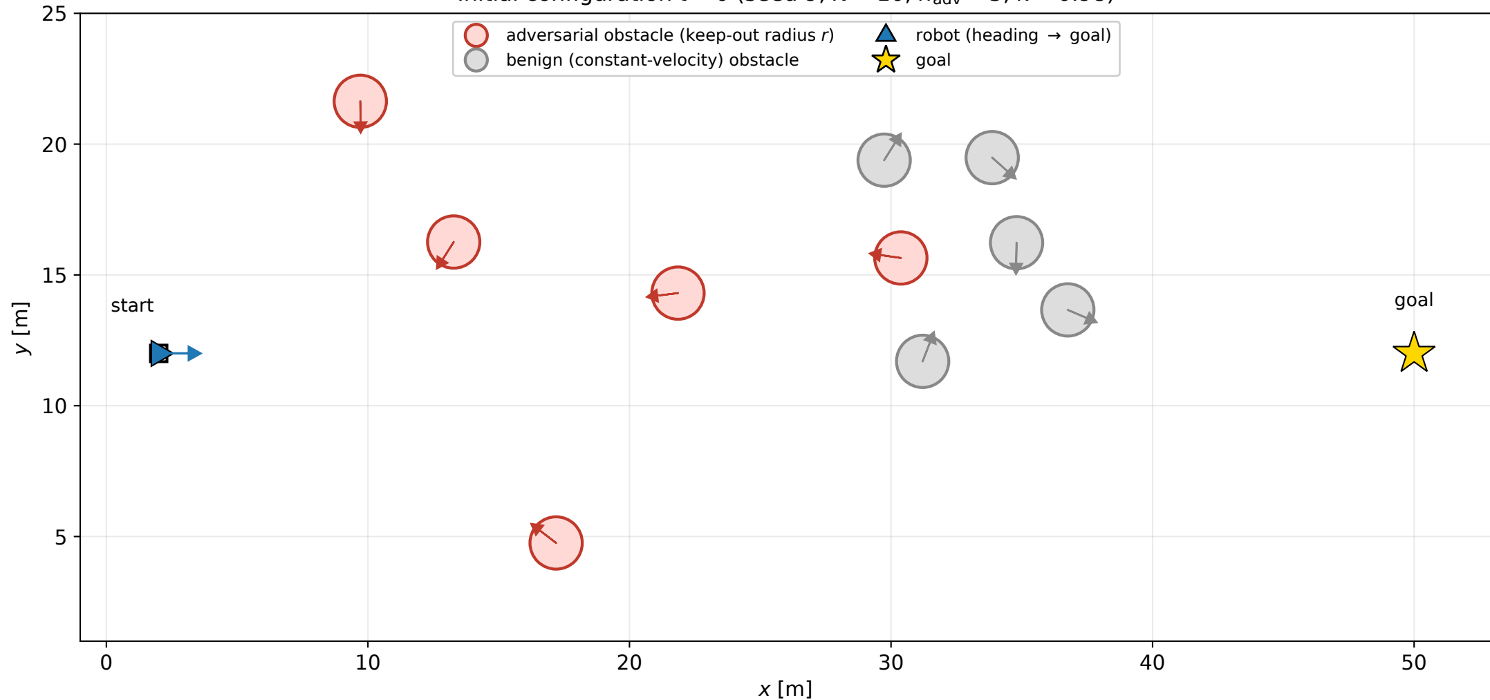
Initial configuration t = 0 (seed 9, N = 10 , n_{\text{adv}} = 5 , \kappa = 0.98 )
