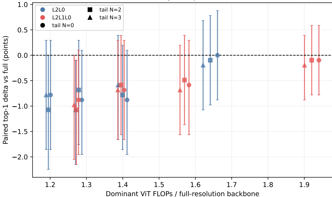
Paired accuracy-compute calibration
