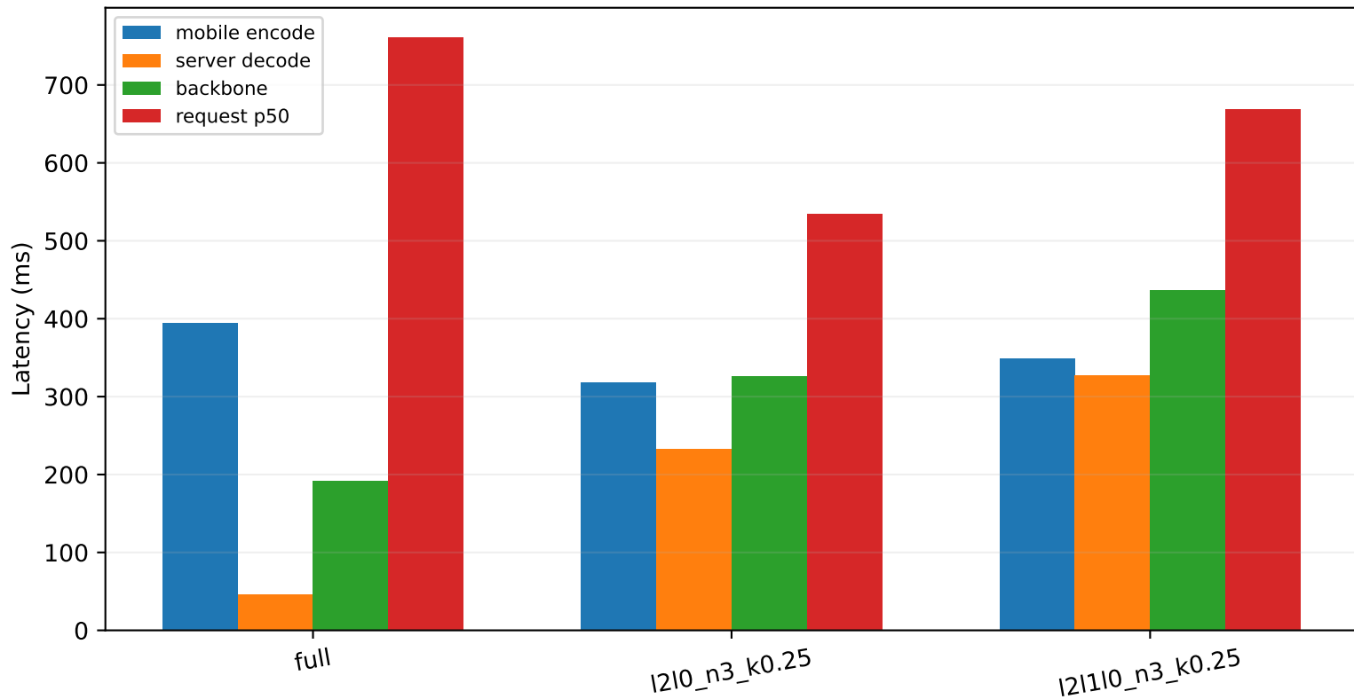
Isolated B200 pipeline components (overlapping)
