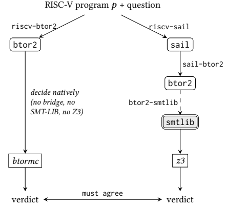
Figure 4. What the bottom block of Table 4 measures: the same question decided along two stacks sharing no decision component after the head (the named residue: emission library, endpoints) — the ISA-prose-derived lowering decided natively by btormc , against the Sail-model-derived lowering through the predicted-grade bridge and Z3. Agreement corroborates the whole diverse segment (Assumption 2); the stated residual shared surface is the BTOR2 emission library and the language-owned endpoint interpreters. The solver-level rows at the top of Table 4 instead decide both sides through the bridge and Z3, sharing everything below the reconvergence.
