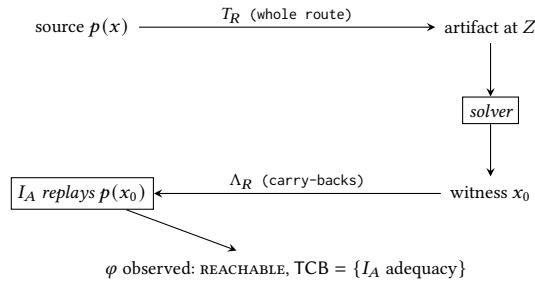
Figure 3. The round trip every case study in Table 6 completes (Theorem 4.6): the witness comes back through the route’s carry-backs and is replayed by the source interpreter. Everything on the way down is a discovery device — a defect in any translator, hub, or the solver can lose the witness, never fake the replay.
