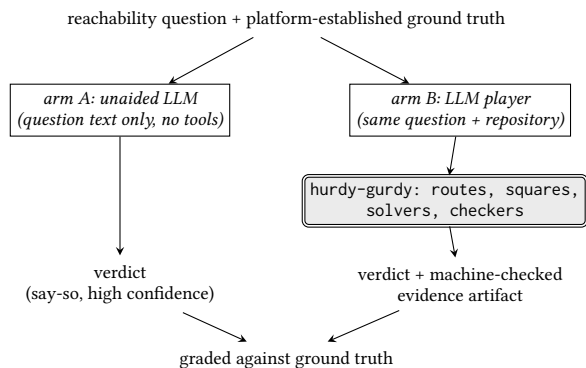
Figure 6. The two-arm player protocol of Table 11: one fresh, context-free agent per question per arm, no retries. Both arms are graded against the same platform-established ground truth; what differs by construction is what the verdict rests on — arm B can take no unchecked step, so every answer carries the evidence artifact of Table 11’s final column.
