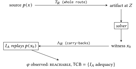
Figure 3. The round trip every case study in Table 6 completes (Theorem 4.8): the witness comes back through the route’s carry-backs and is replayed by the source interpreter. Everything on the way down is a discovery device — a defect in any translator, hub, or the solver can lose the witness, never fake the replay.
