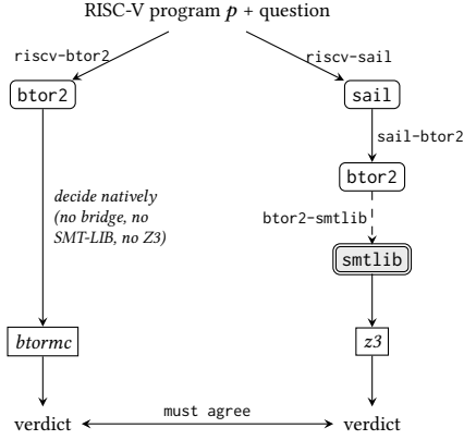
Figure 2. What the bottom block of Table 4 measures: the same question decided along two stacks sharing no decision component after the head (the named residue: emission library, endpoints) — the ISA-prose-derived lowering decided natively by btormc , against the Sail-model-derived lowering through the predicted-grade bridge and Z3. Agreement corroborates the whole diverse segment (Assumption 2); the stated residual shared surface is the BTOR2 emission library and the language-owned endpoint interpreters. The solver-level rows at the top of Table 4 instead decide both sides through the bridge and Z3, sharing everything below the reconvergence.
