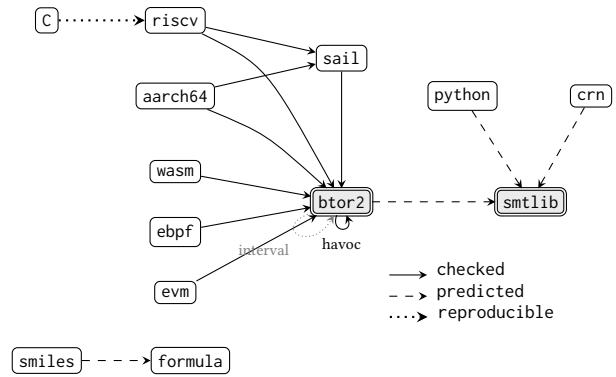
Figure 1. The registry: 13 languages (nodes; the two reasoning hubs shaded) and 15 registered pairs (edges), each carrying its declared grade. The two loops on the BTOR2 hub are the abstraction endo-pairs of the direction axis (§3.4): btor2-havoc , built , and — dotted — btor2-interval , registered as a brief. The evaluation of Section 6 covers the thirteen pairs built at its snapshot. RISC-V and AArch64 each reach BTOR2 twice — directly (manual-derived) and through Sail (formal-model-derived) — the independently derived branches Assumption 2 requires, each leg’s semantic artifact declared per pair; the dashed btor2 → smtlib bridge is the shared suffix that the disjoint-decision runs of §6.2 remove from the corroborating pair.
