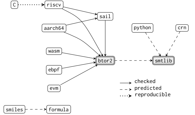
Figure 1. The registry at the snapshot: 13 languages (nodes; the two reasoning hubs shaded), 13 pairs (edges), each edge carrying its declared grade. RISC-V and AArch64 each reach BTOR2 twice — directly (manual-derived) and through Sail (formal-model-derived) — the independently derived branches Assumption 2 requires; the dashed btor2 → smtlib bridge is the shared suffix that the disjoint-decision runs of §6.2 remove from the corroborating pair.
