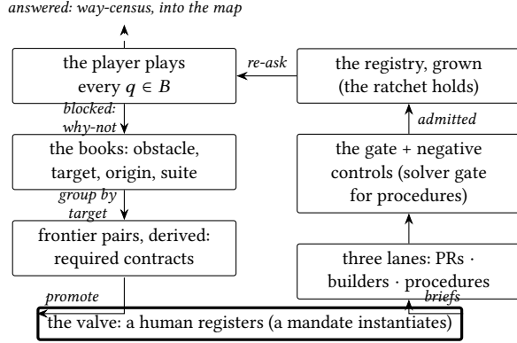
Figure 3. One loop iteration. Demand descends on the left — every failure a typed record on the books, aggregating into frontier pairs — and supply ascends on the right, but only through the valve at the bottom: registration is the one human act (or its earned, revocable mandate). The two planes meet nowhere else: answers never write, growth never answers. Monotonicity (Theorem 5.2) makes the cycle a ratchet, never a treadmill.
