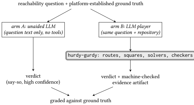
Figure 6. The two-arm player protocol of Table 10: one fresh, context-free agent per question per arm, no retries. Both arms are graded against the same platform-established ground truth; what differs by construction is what the verdict rests on — arm B can take no unchecked step, so every answer carries the evidence artifact of Table 10’s final column.
