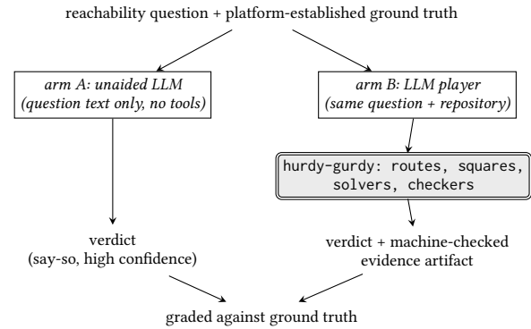
Figure 6. The two-arm player protocol of Table 11: one fresh, context-free agent per question per arm, no retries. Both arms are graded against the same platform-established ground truth; what differs by construction is what the verdict rests on — arm B can take no unchecked step, so every answer carries the evidence artifact of Table 11’s final column.
