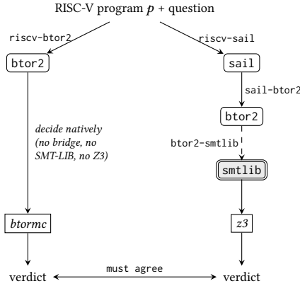
Figure 2. What the bottom block of Table 4 measures: the same question decided along two stacks that share nothing after the head — the ISA-prose-derived lowering decided natively by btormc , against the Sail-model-derived lowering through the predicted-grade bridge and Z3. Agreement corroborates the whole diverse segment (Assumption 2); the stated residual shared surface is the BTOR2 emission library and the language-owned endpoint interpreters. The solver-level rows at the top of Table 4 instead decide both sides through the bridge and Z3, sharing everything below the reconvergence.
