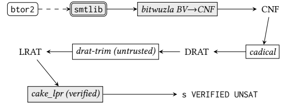
Figure 4. The pipeline Table 7 evaluates: the query is bit-blasted to CNF, cadical’s DRAT refutation is elaborated by drat-trim — an untrusted step that can only fail the re-check, never fake a pass — and cake_lpr, the formally verified checker, re-validates the LRAT against the CNF from scratch. Shaded is what stays in the verdict’s TCB: the bit-blast and the verified checker; the three agreeing engines and the elaborator are discovery devices.
