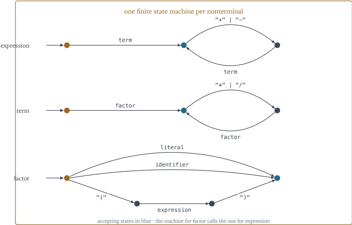
a context-free grammar, one FSM per rule, and a stack
