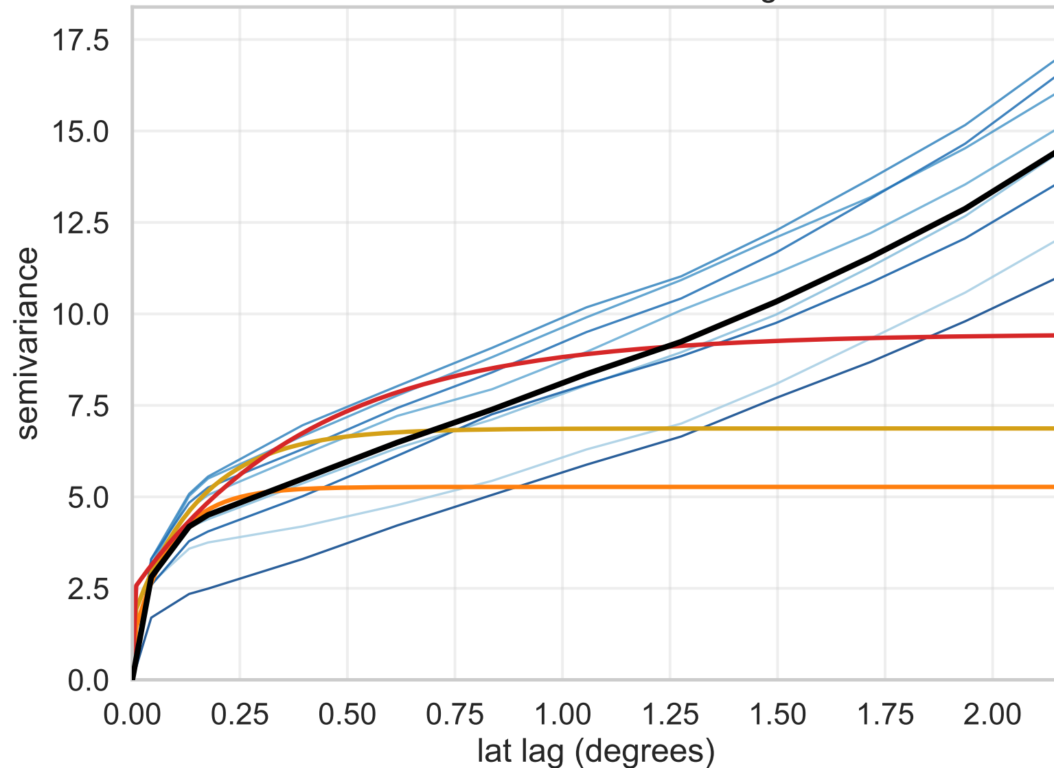
Latitude-direction semivariogram
