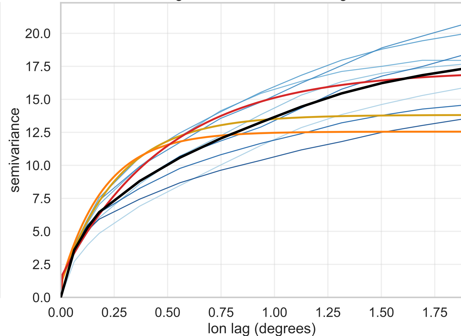
Longitude-direction semivariogram
