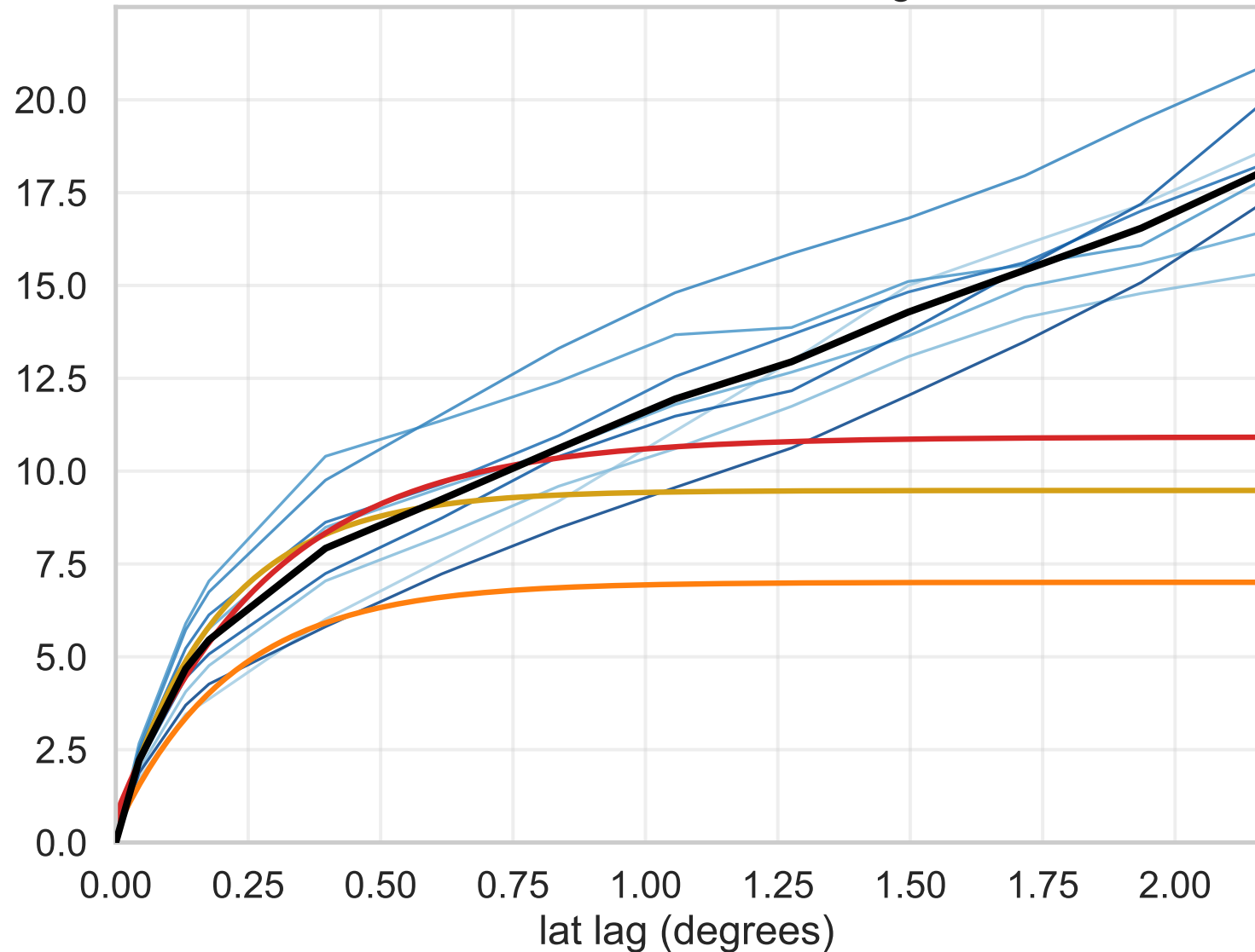
Latitude-direction semivariogram
