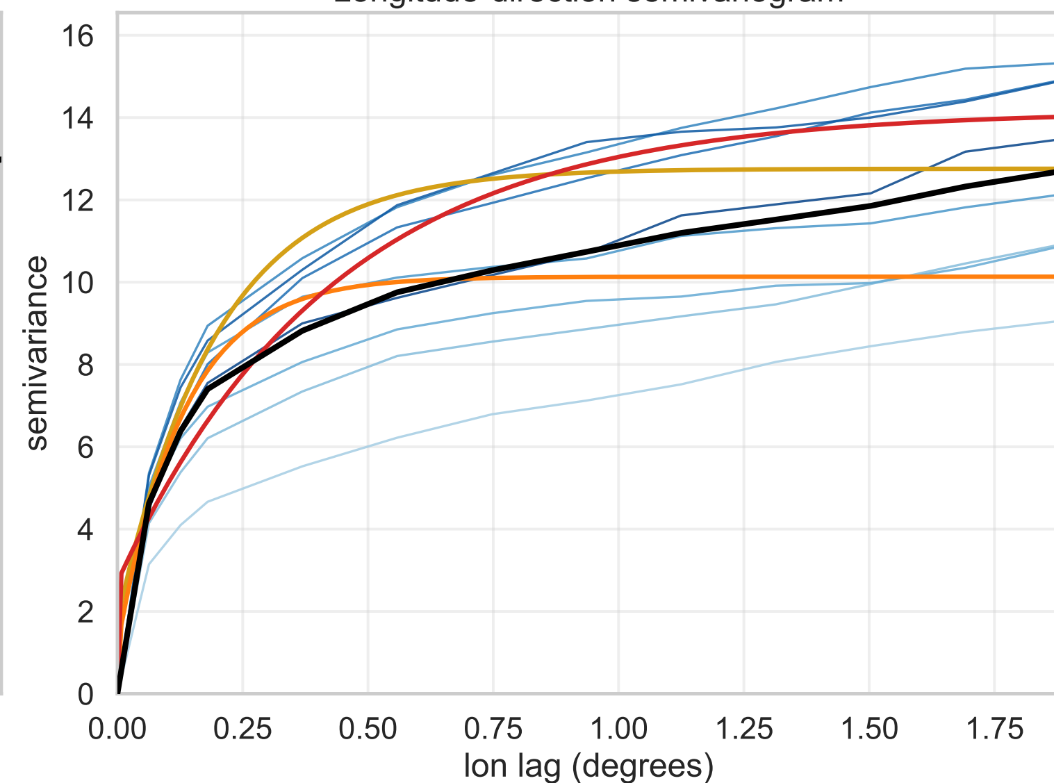
Longitude-direction semivariogram
