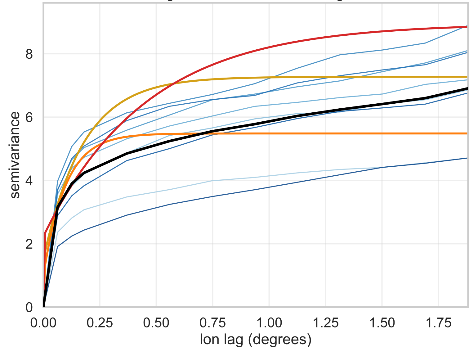
Longitude-direction semivariogram
