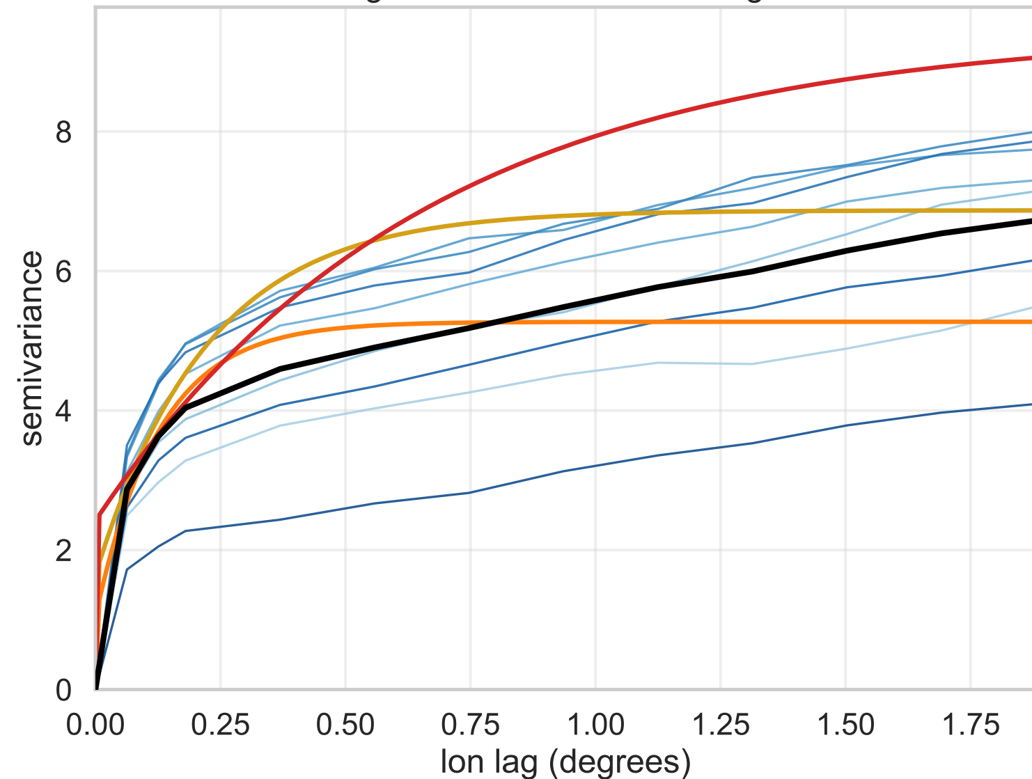
Longitude-direction semivariogram
