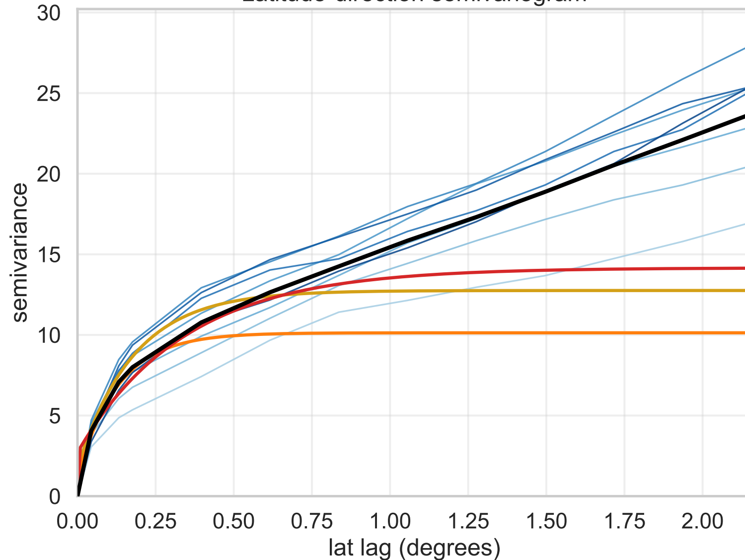
Latitude-direction semivariogram
