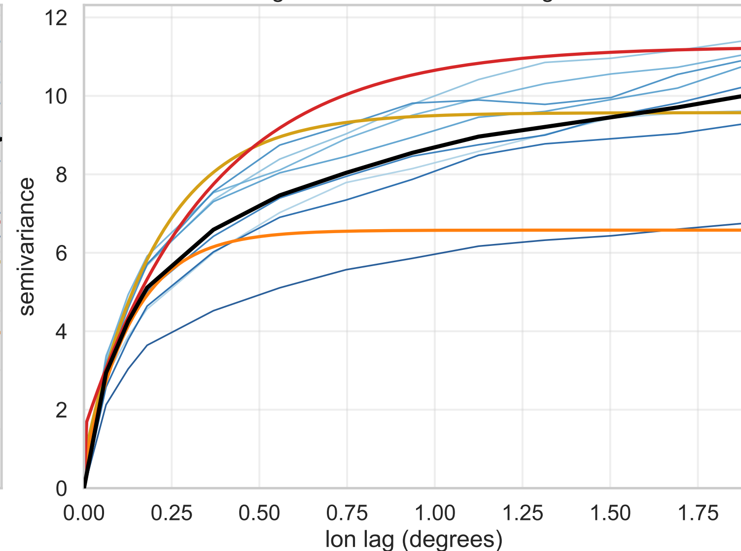
Longitude-direction semivariogram
