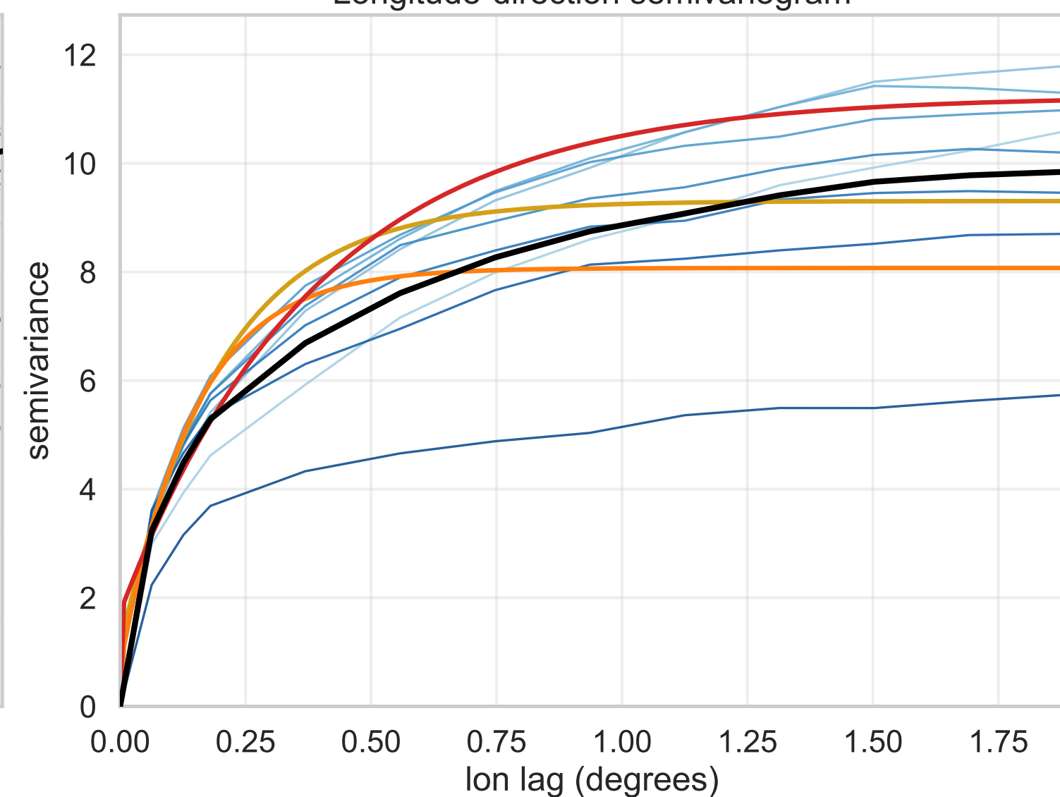
Longitude-direction semivariogram
