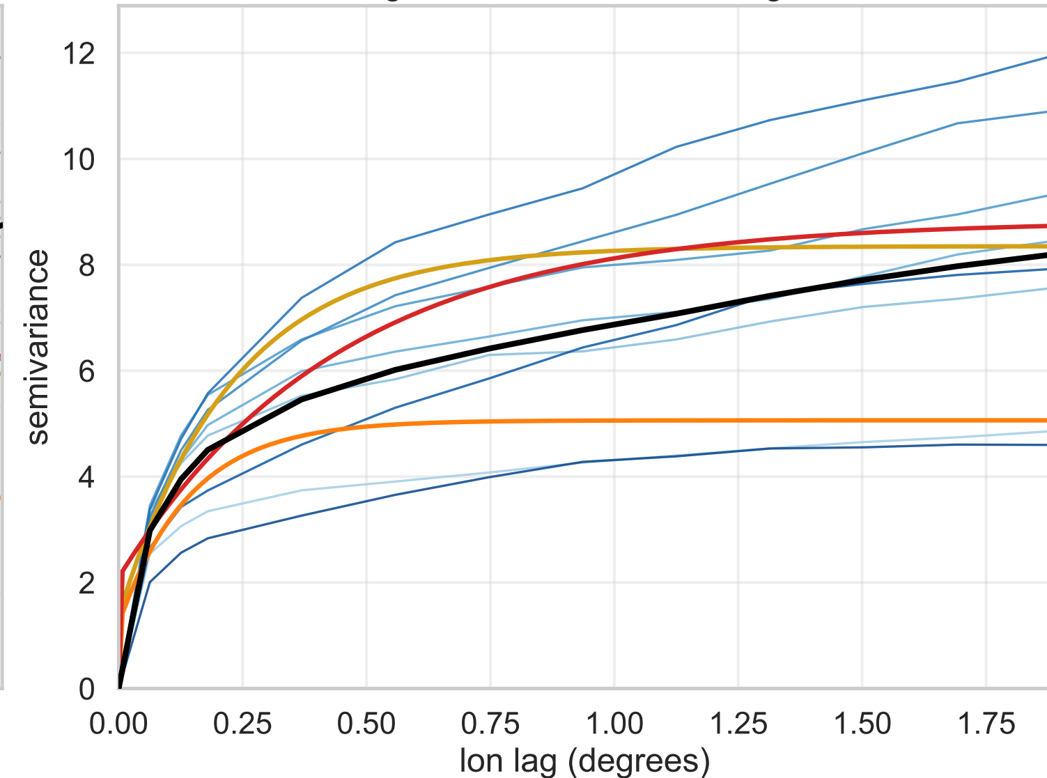
Longitude-direction semivariogram
