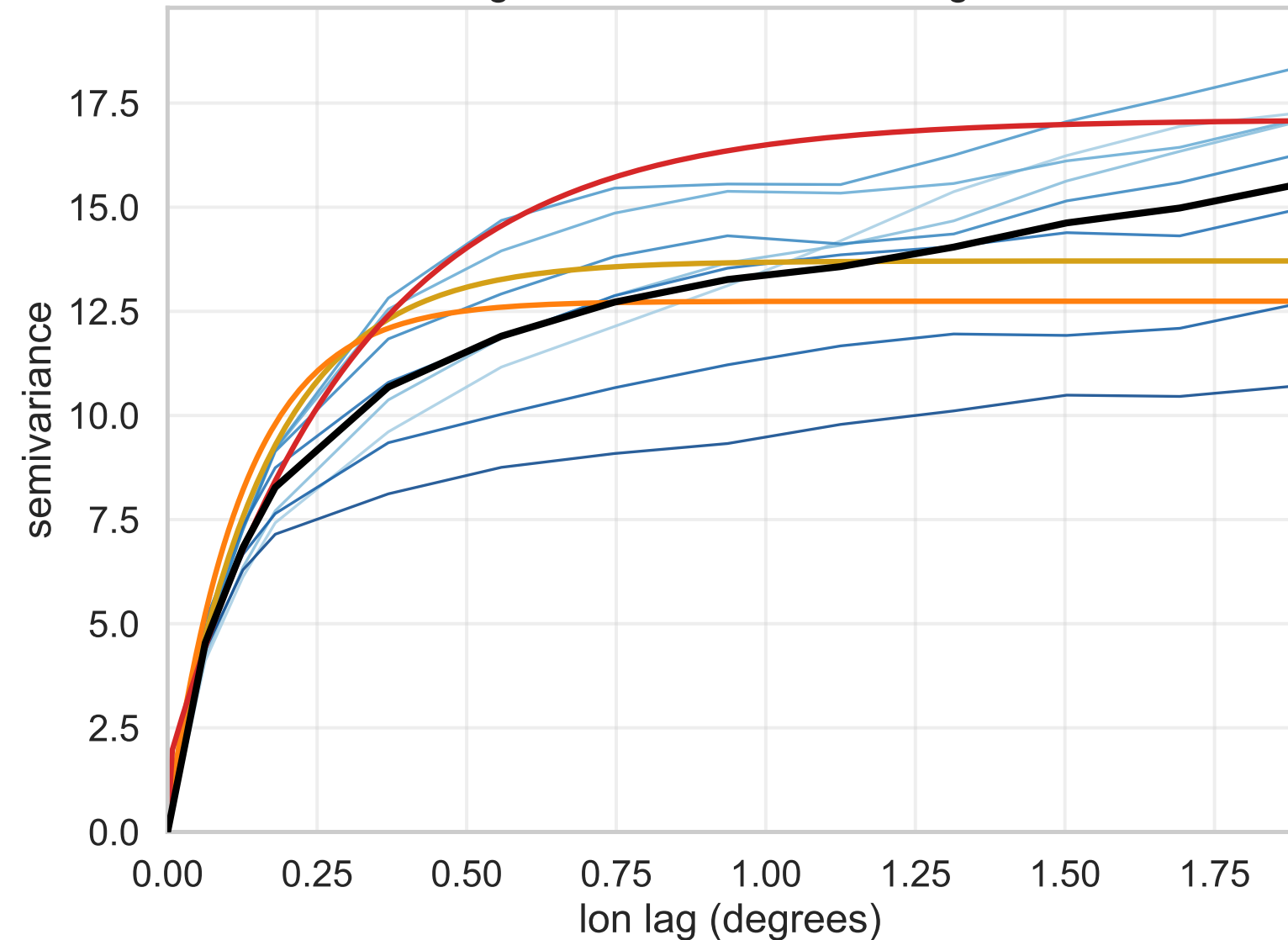
Longitude-direction semivariogram
