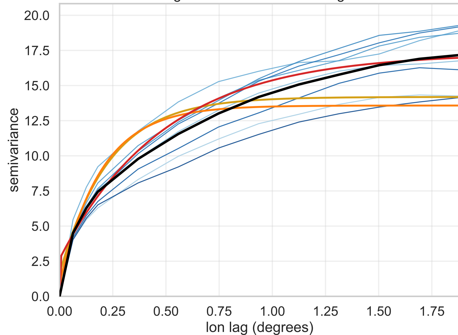
Longitude-direction semivariogram
