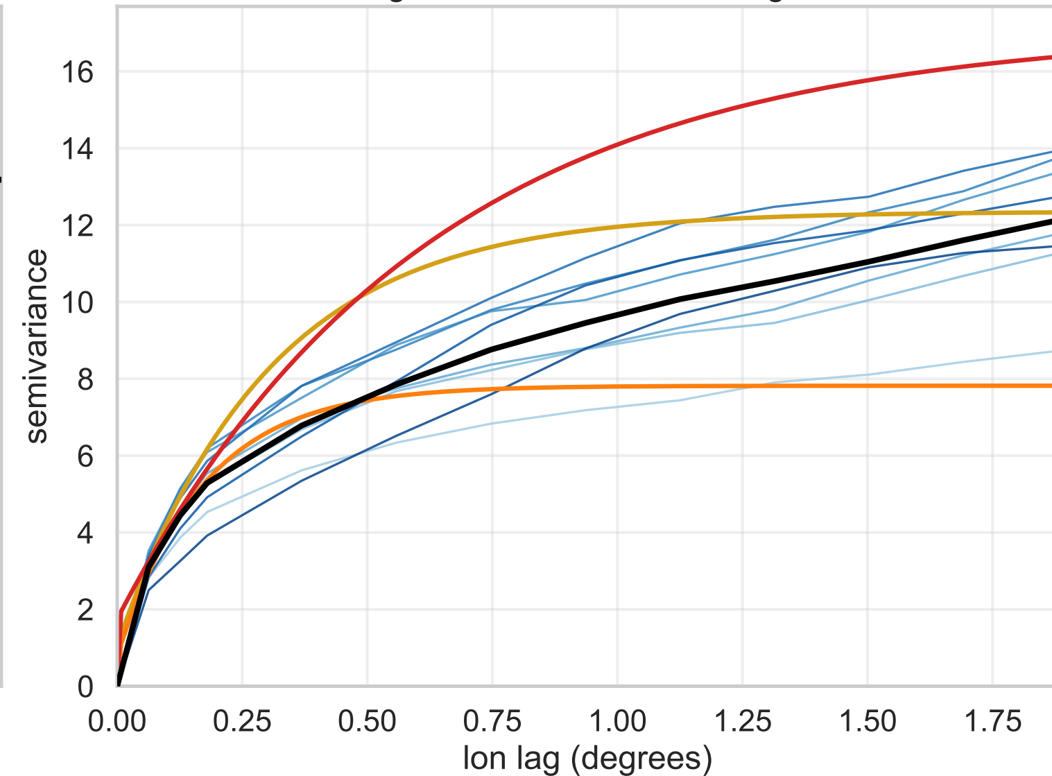
Longitude-direction semivariogram
