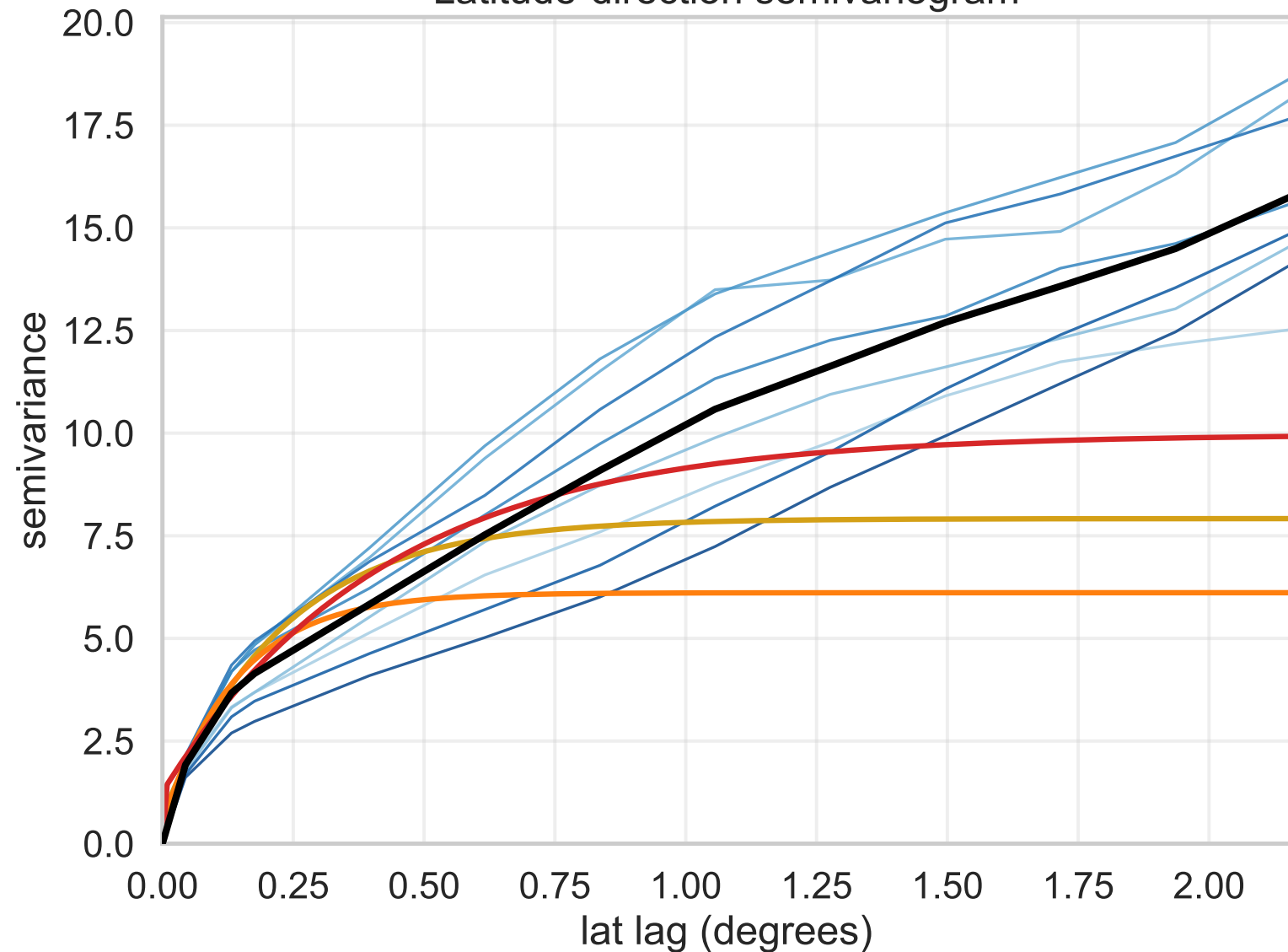
Latitude-direction semivariogram
