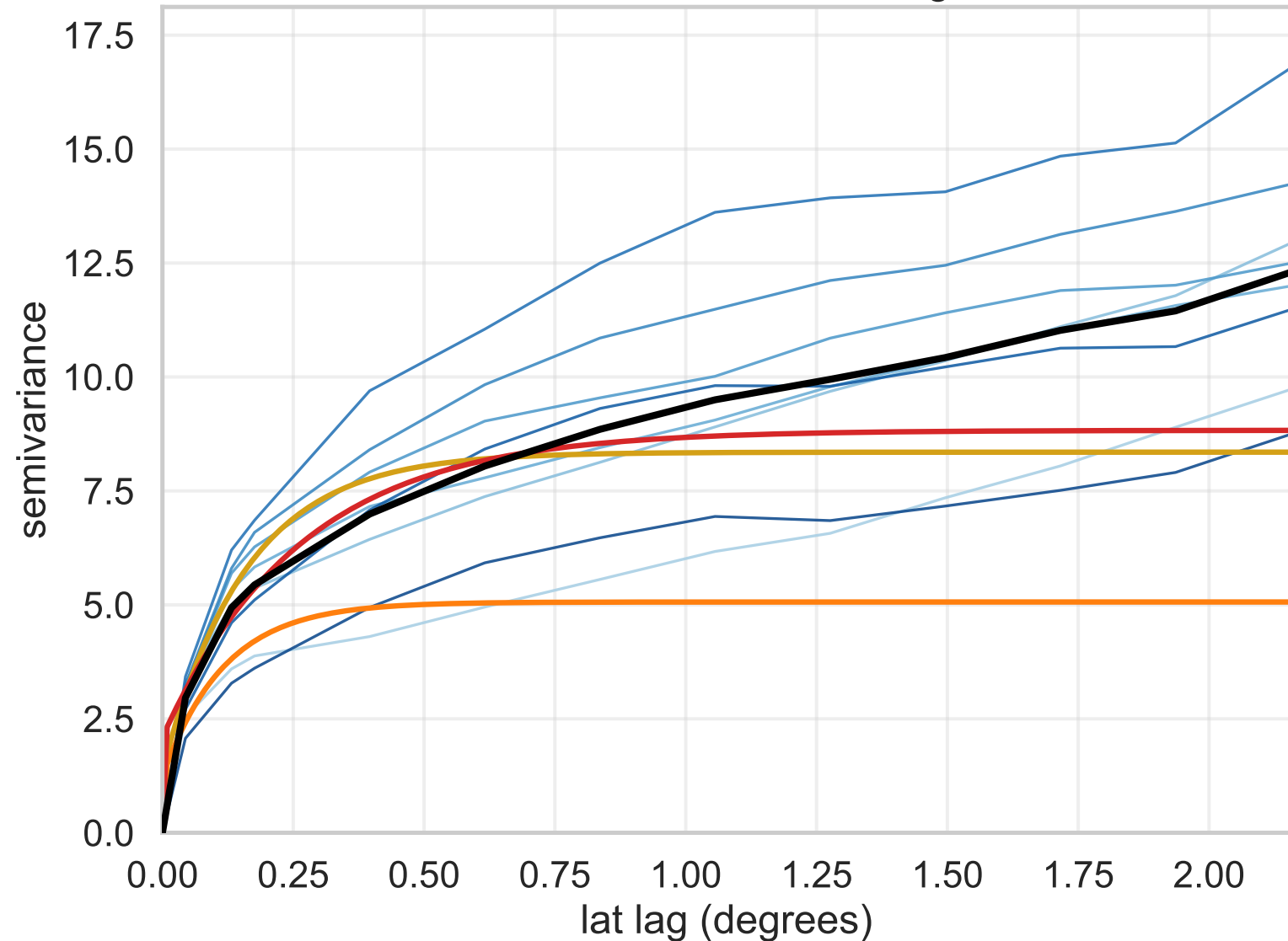
Latitude-direction semivariogram
