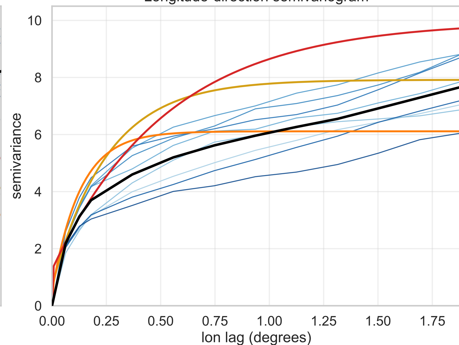
Longitude-direction semivariogram
