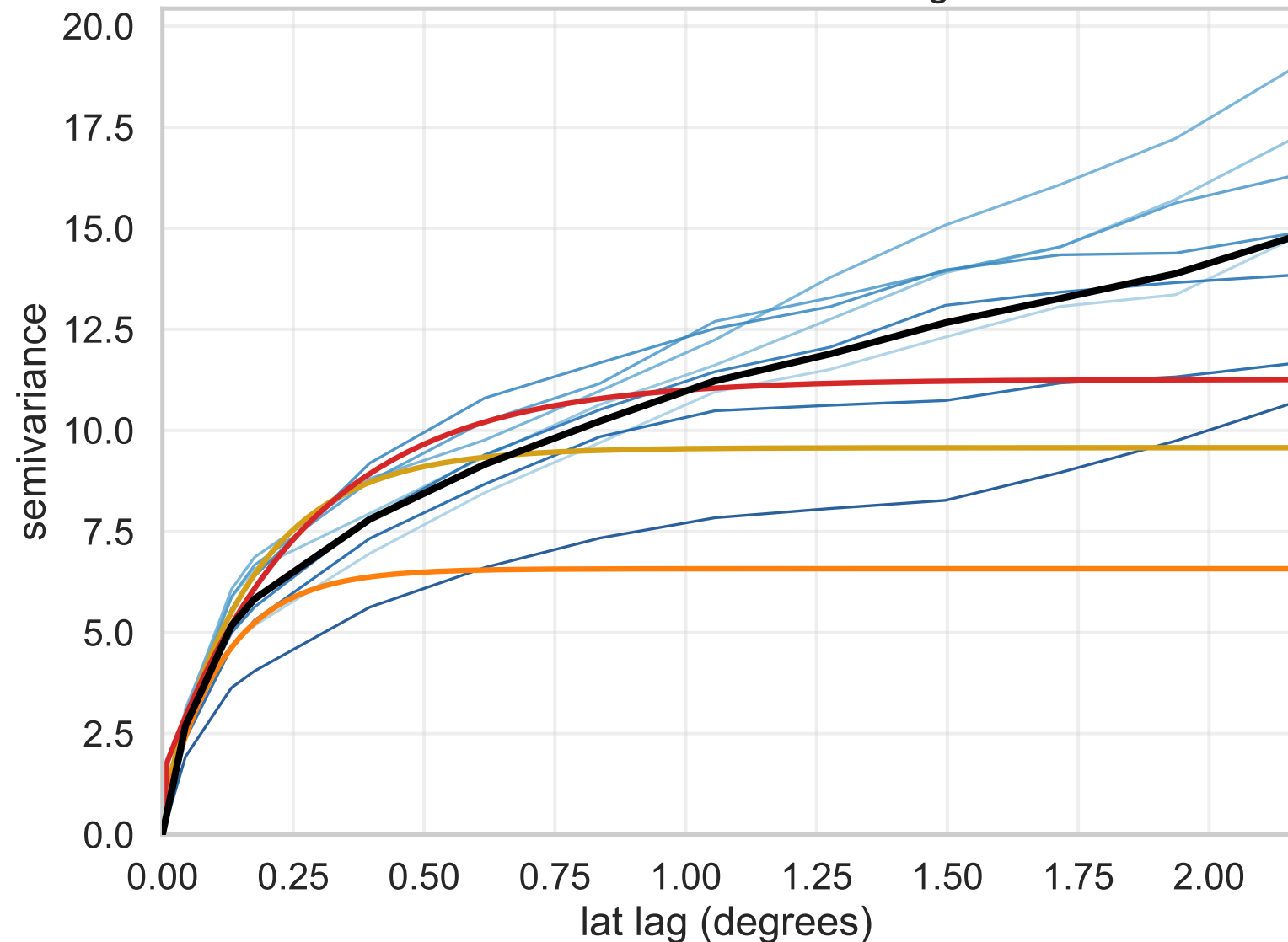
Latitude-direction semivariogram
