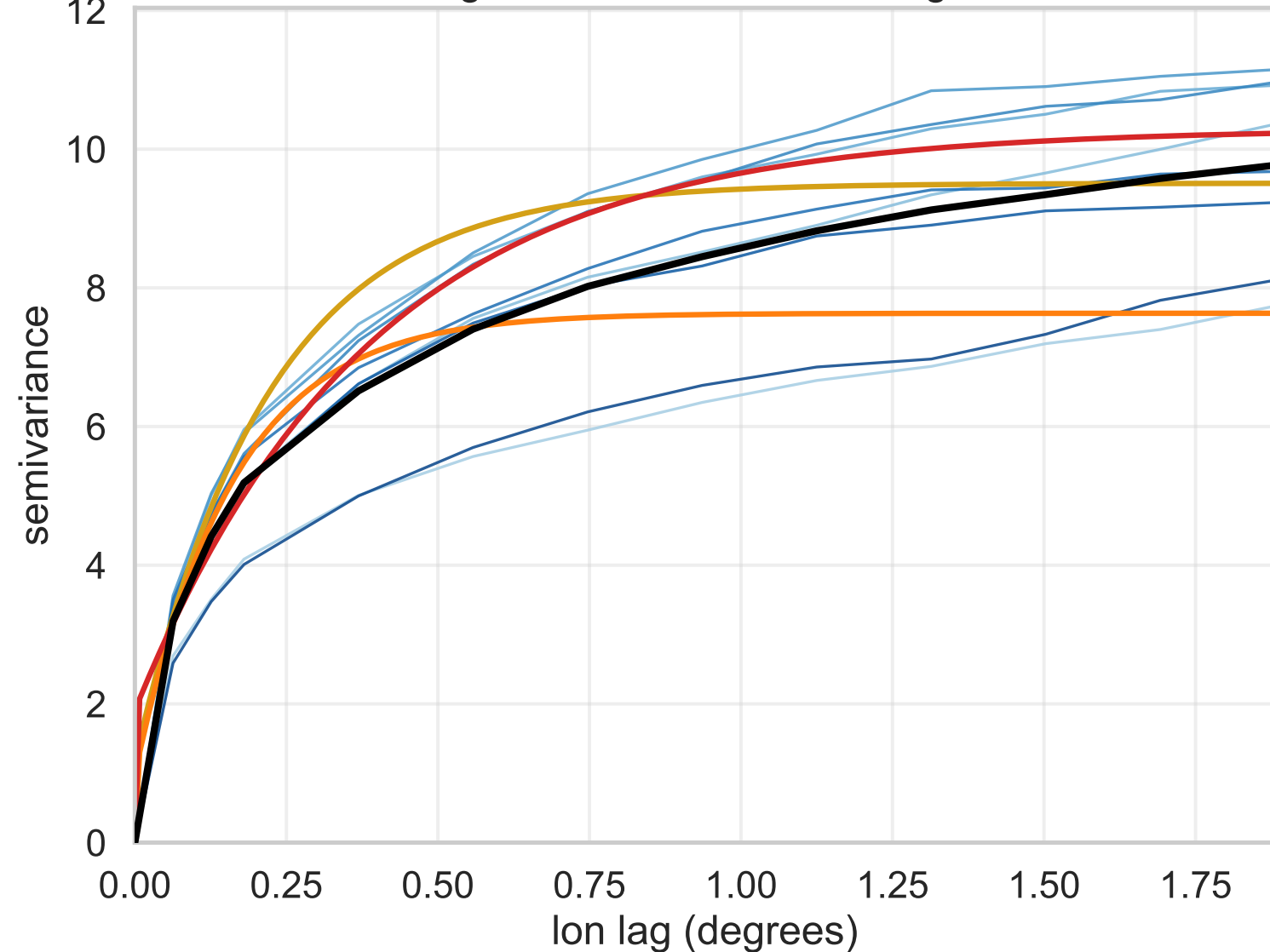
Longitude-direction semivariogram
