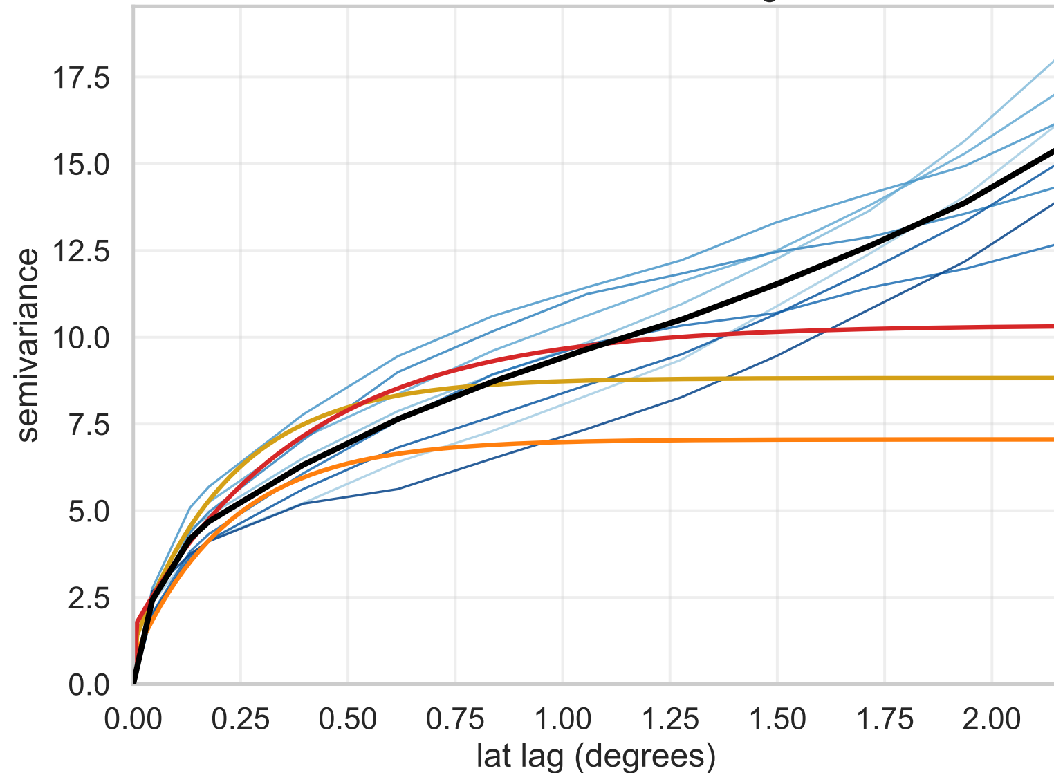
Latitude-direction semivariogram
