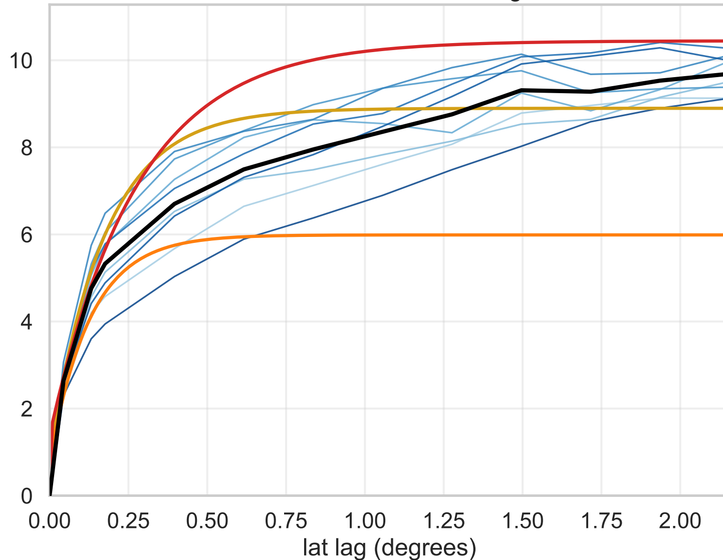
Latitude-direction semivariogram
