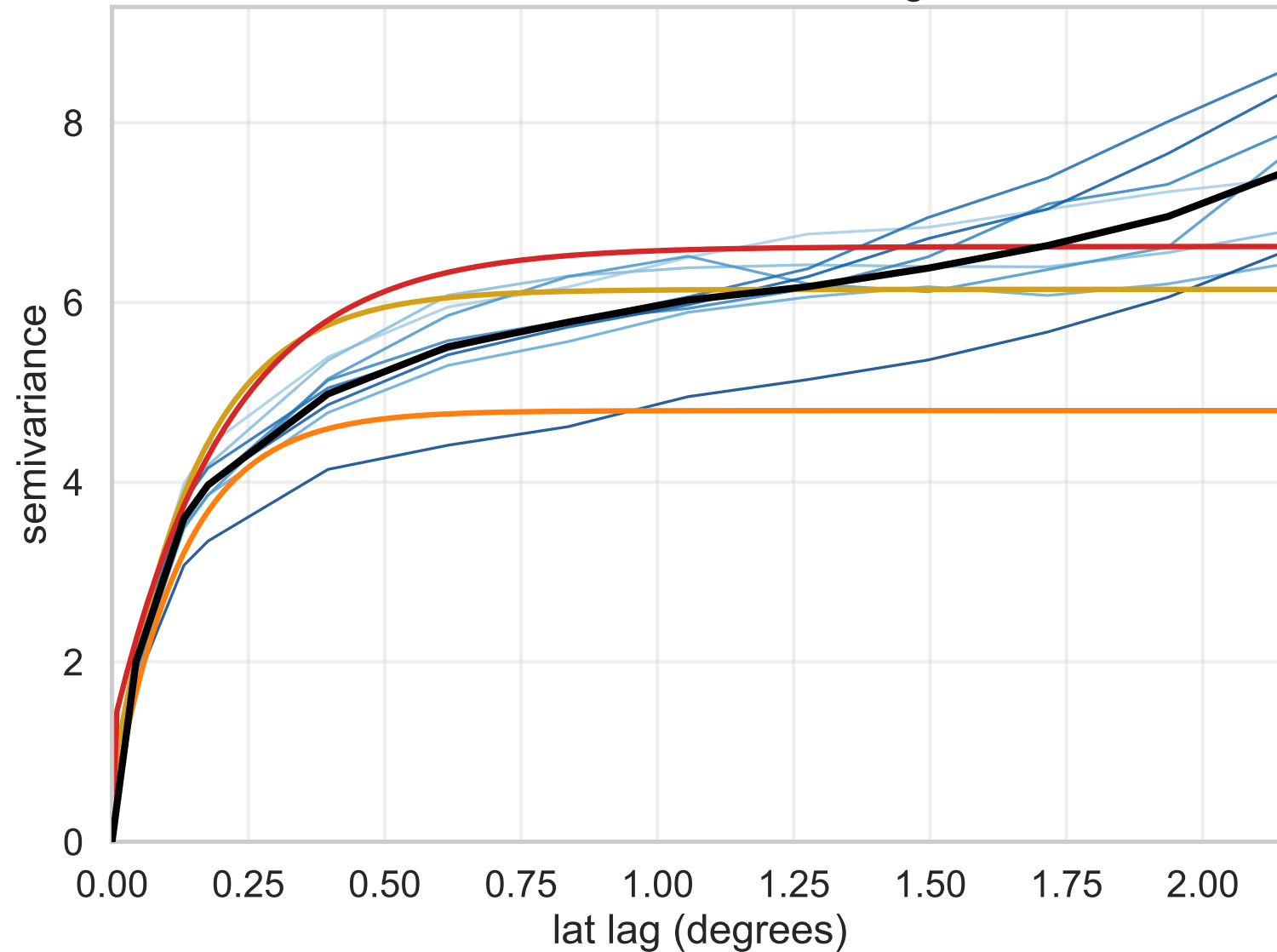
Latitude-direction semivariogram
