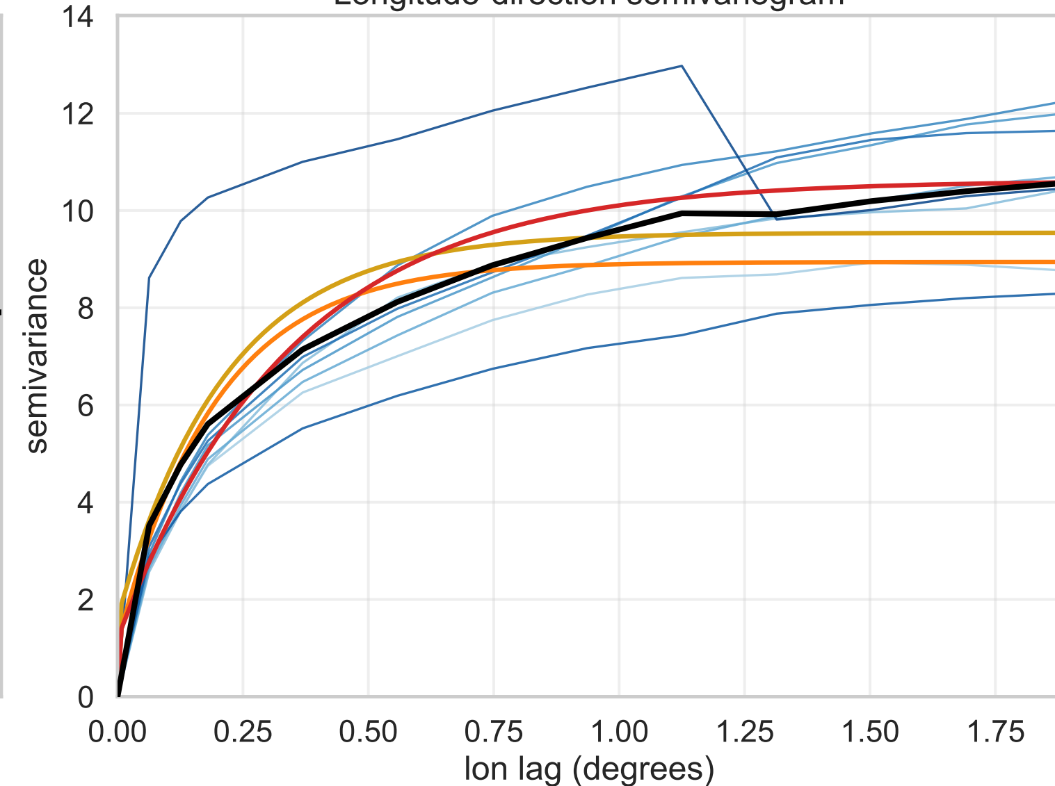
Longitude-direction semivariogram
