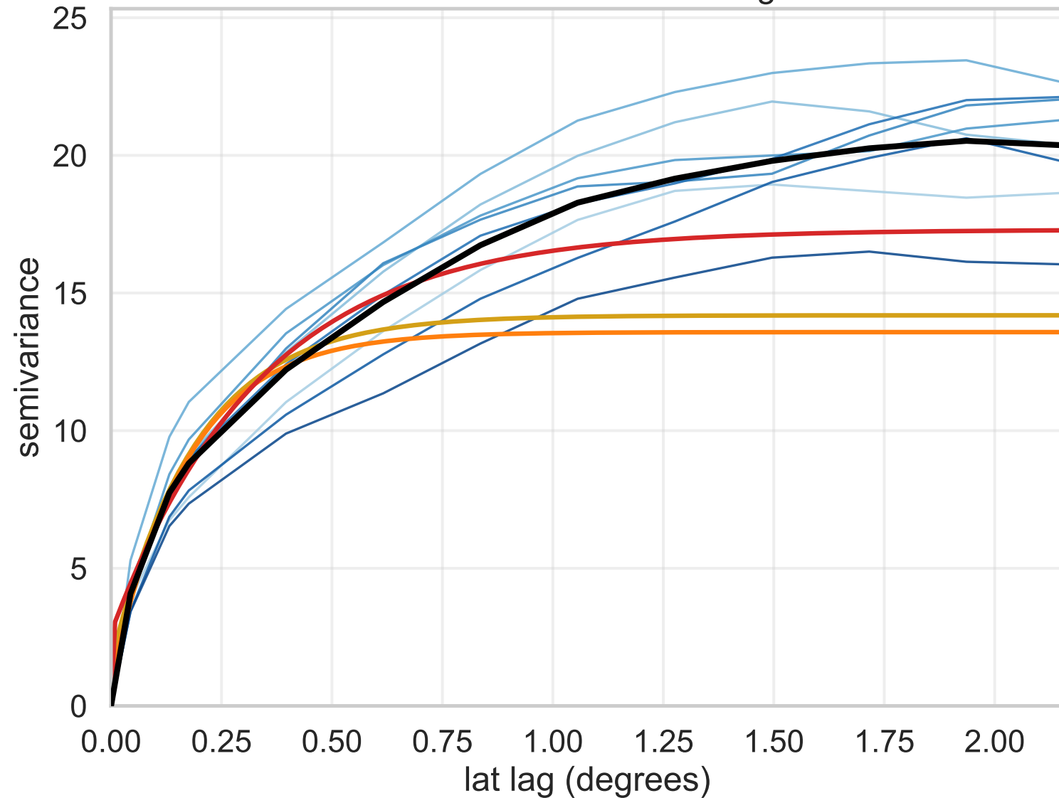
Latitude-direction semivariogram
