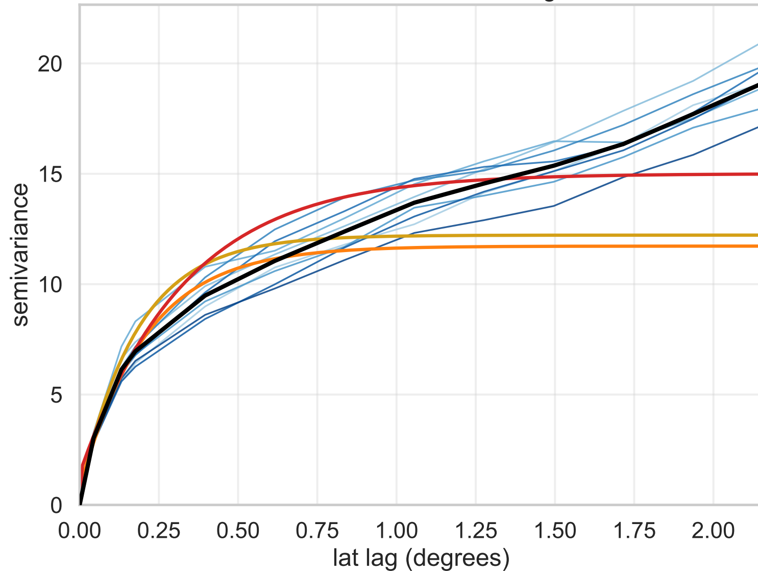
Latitude-direction semivariogram
