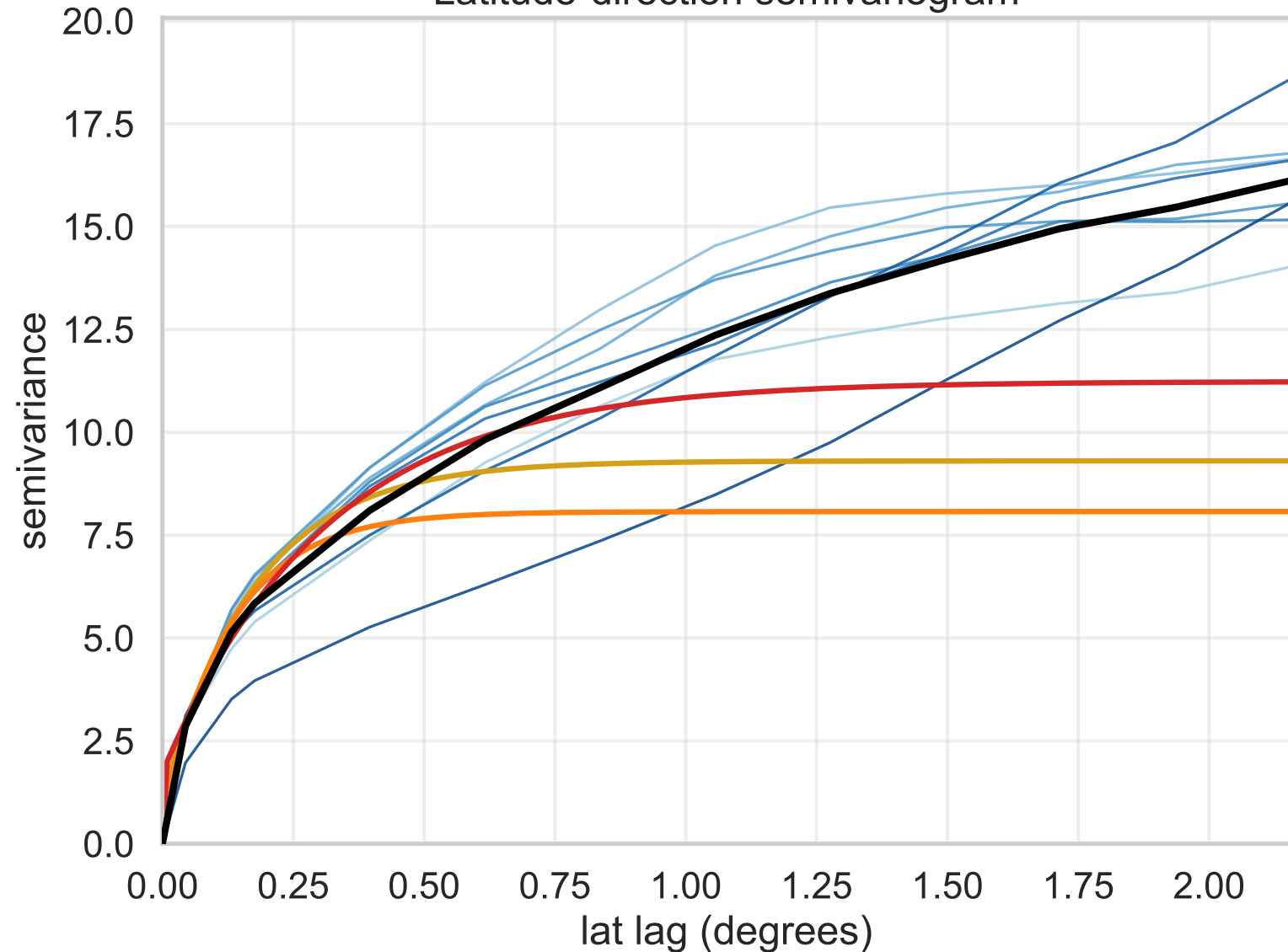
Latitude-direction semivariogram
