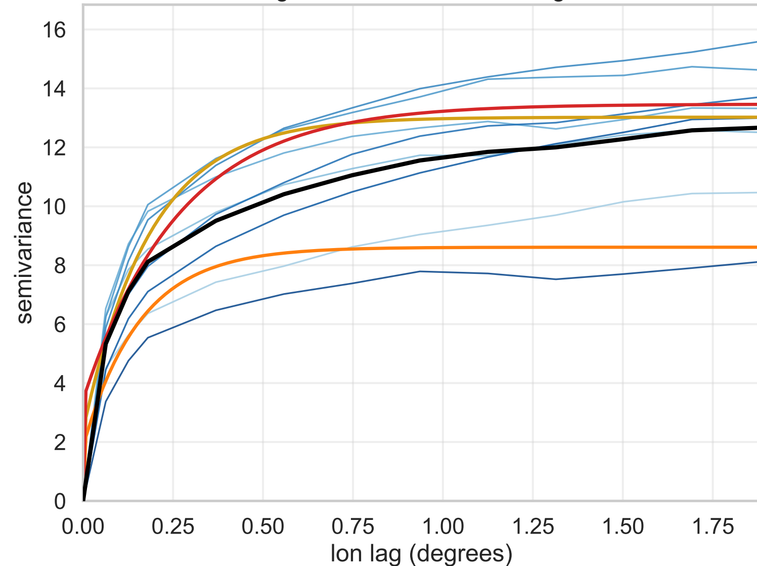
Longitude-direction semivariogram
