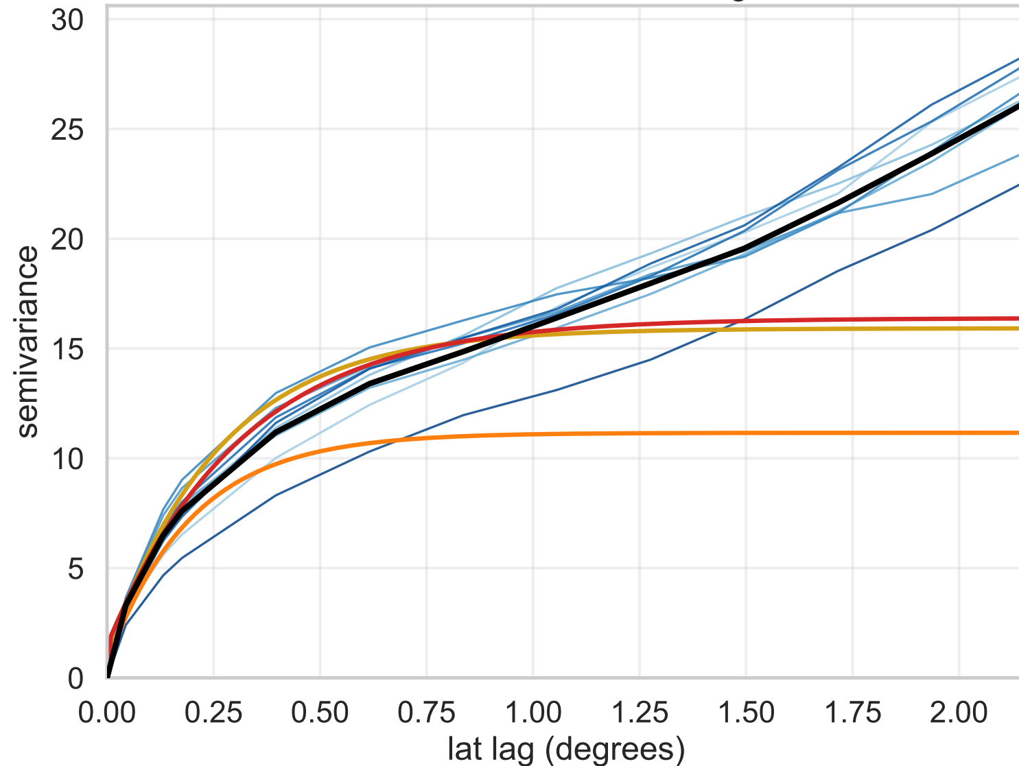
Latitude-direction semivariogram
