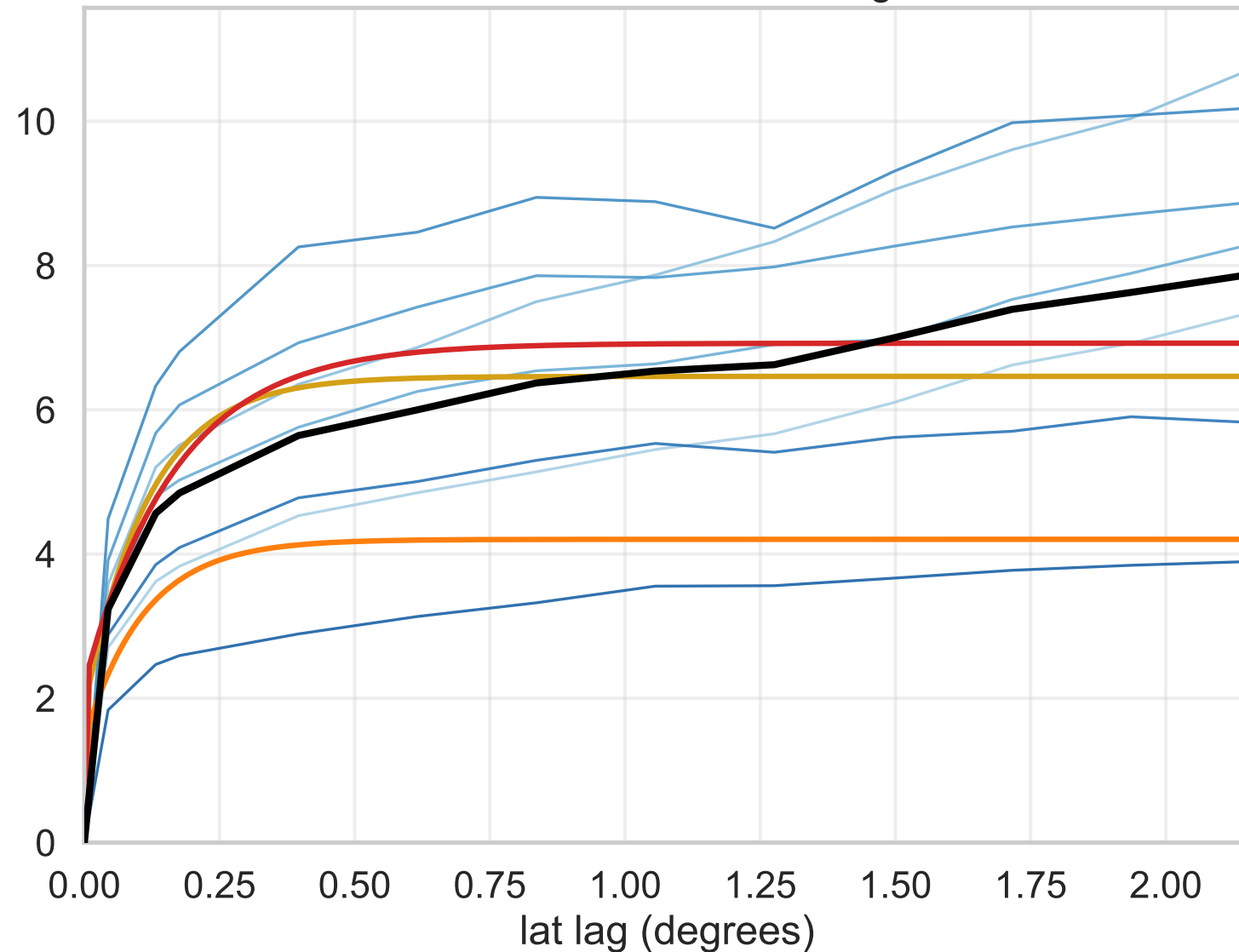
Latitude-direction semivariogram
