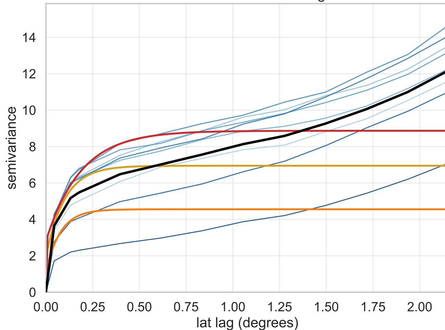
Latitude-direction semivariogram
