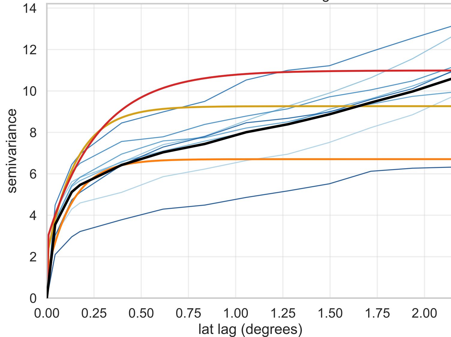
Latitude-direction semivariogram
