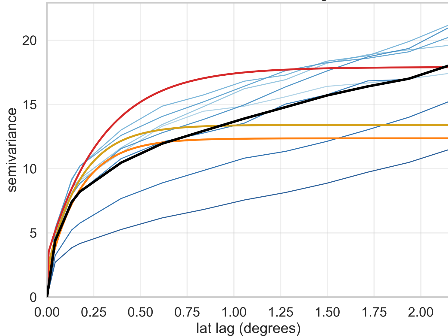
Latitude-direction semivariogram
