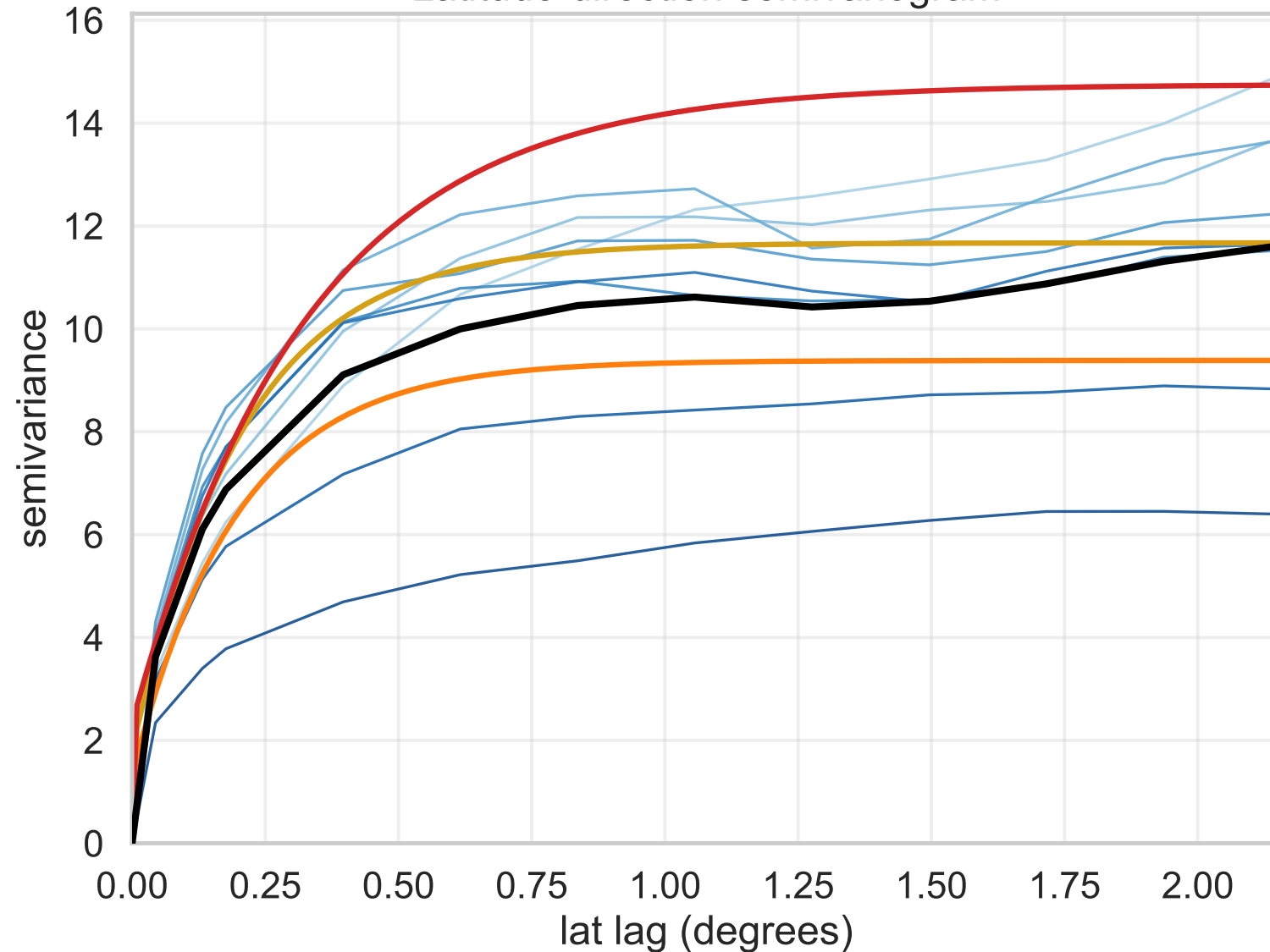
Latitude-direction semivariogram
