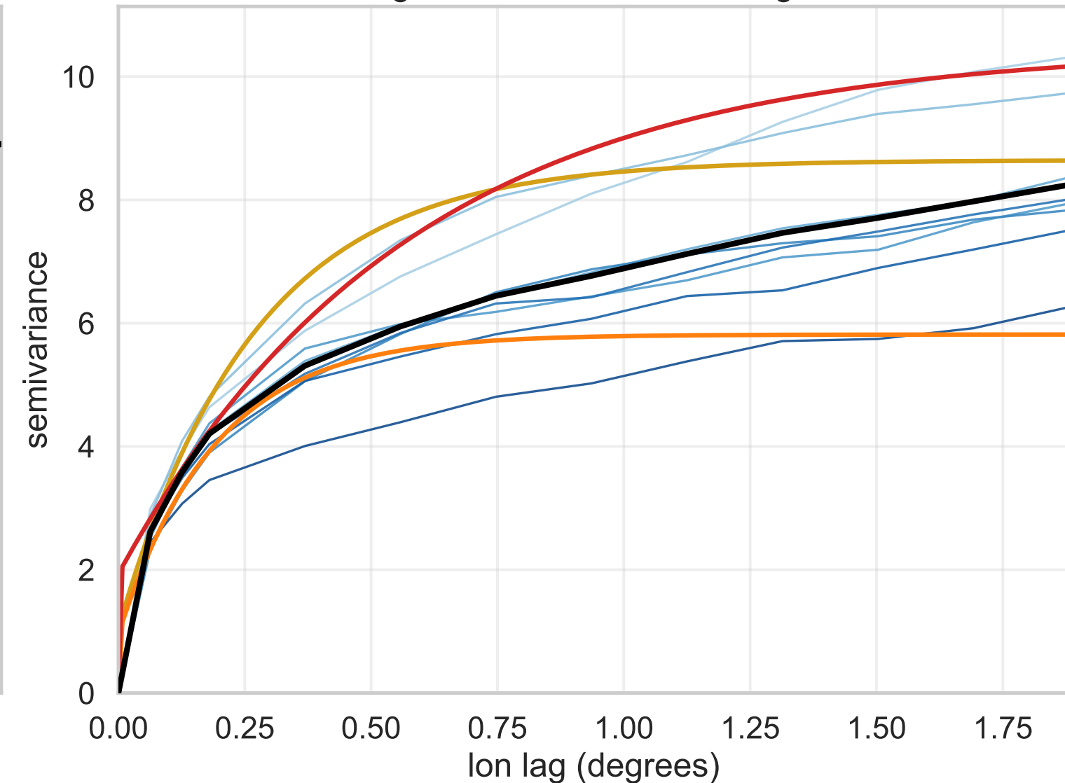
Longitude-direction semivariogram
