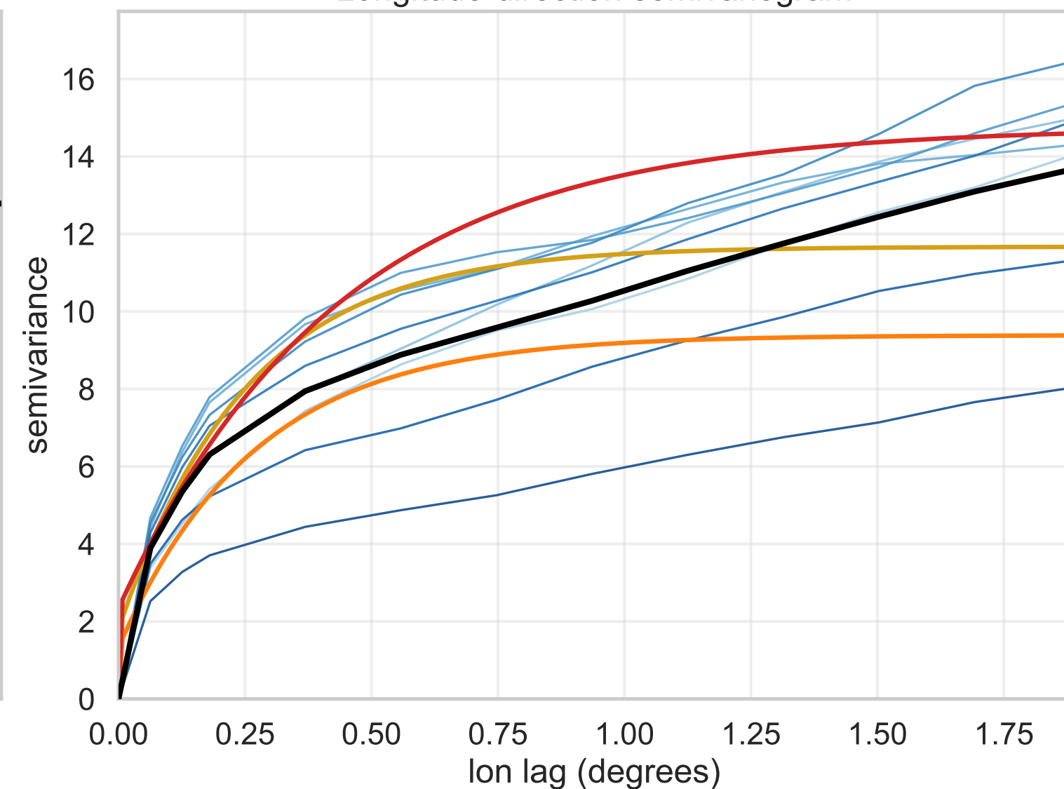
Longitude-direction semivariogram
