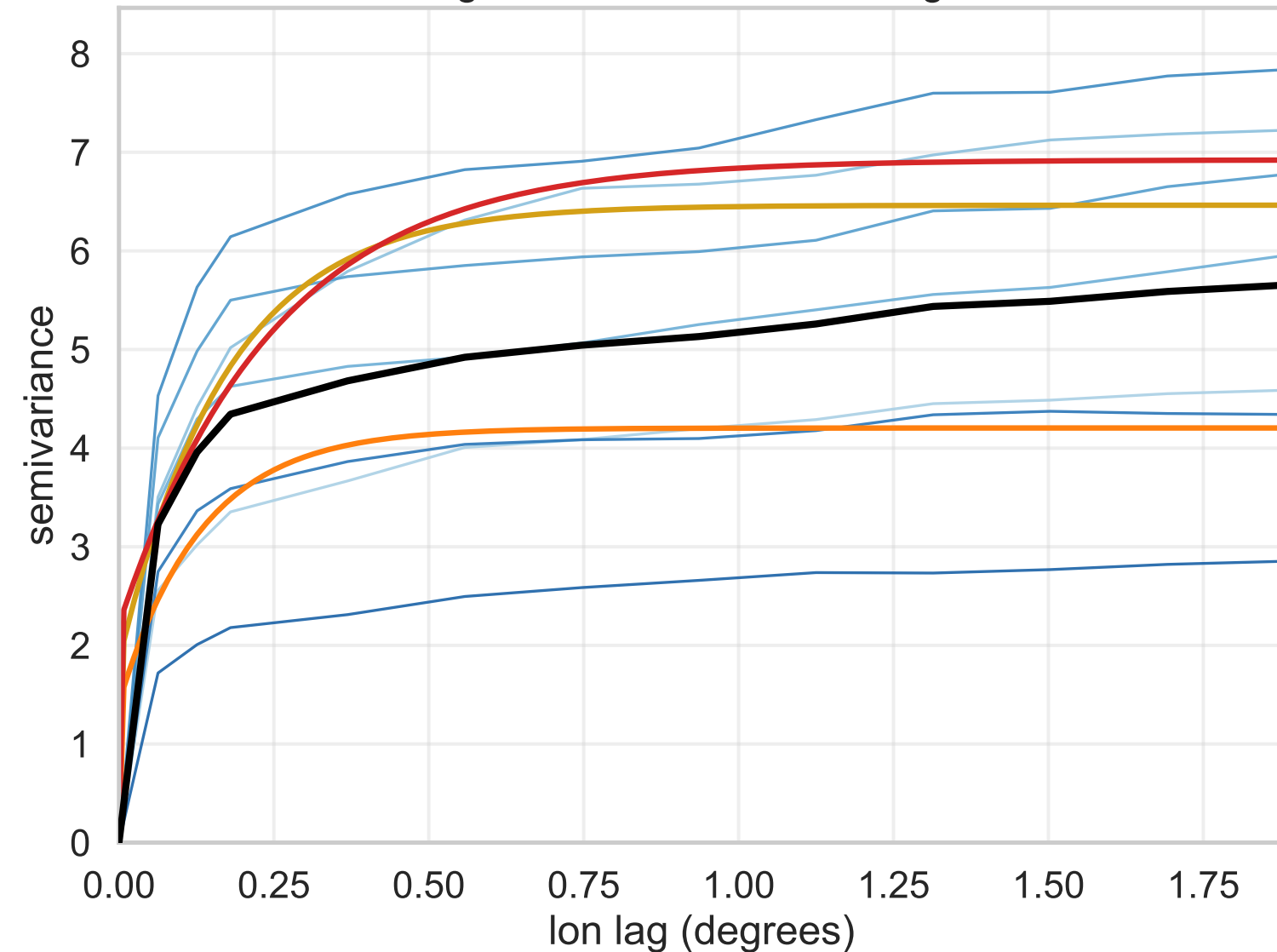
Longitude-direction semivariogram
