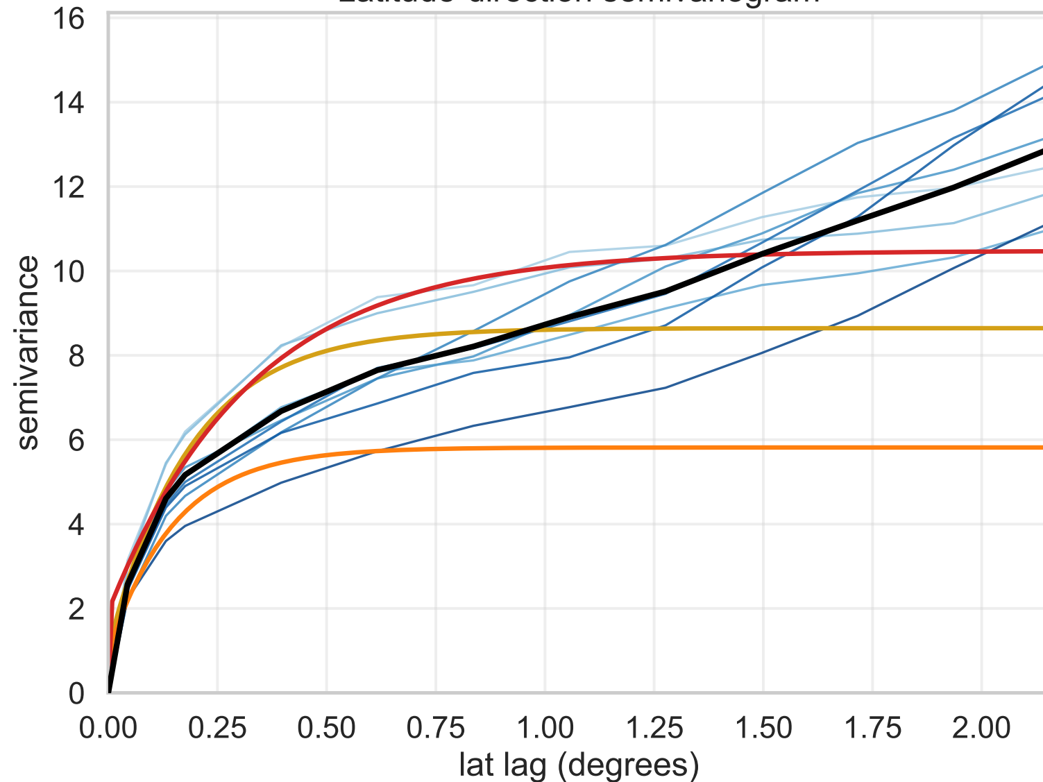
Latitude-direction semivariogram
