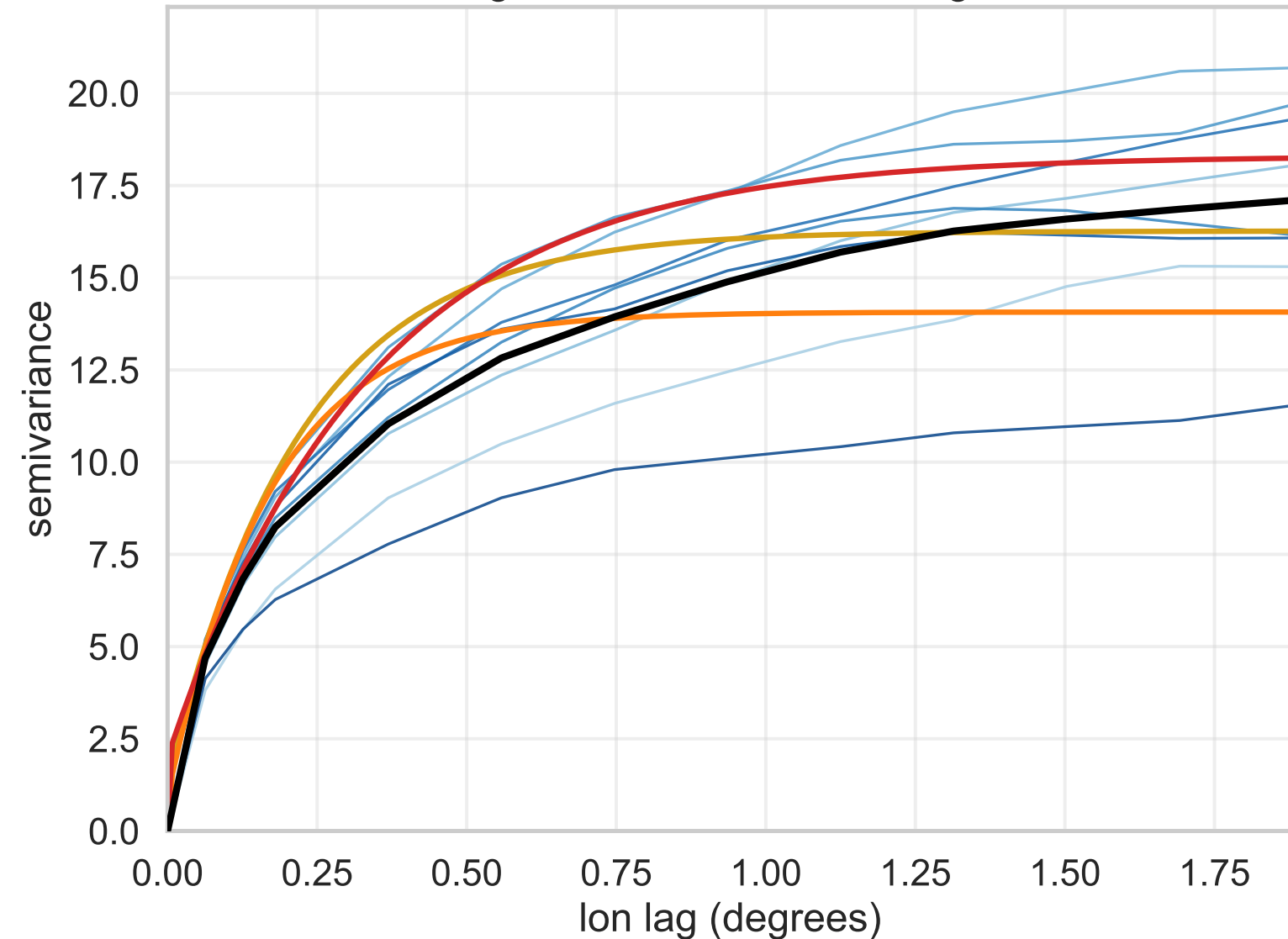
Longitude-direction semivariogram
