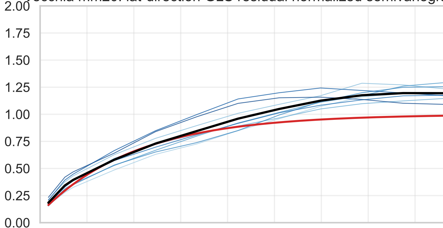
Debiased Whittle: lat-direction GLS residual normalized semivariogram
