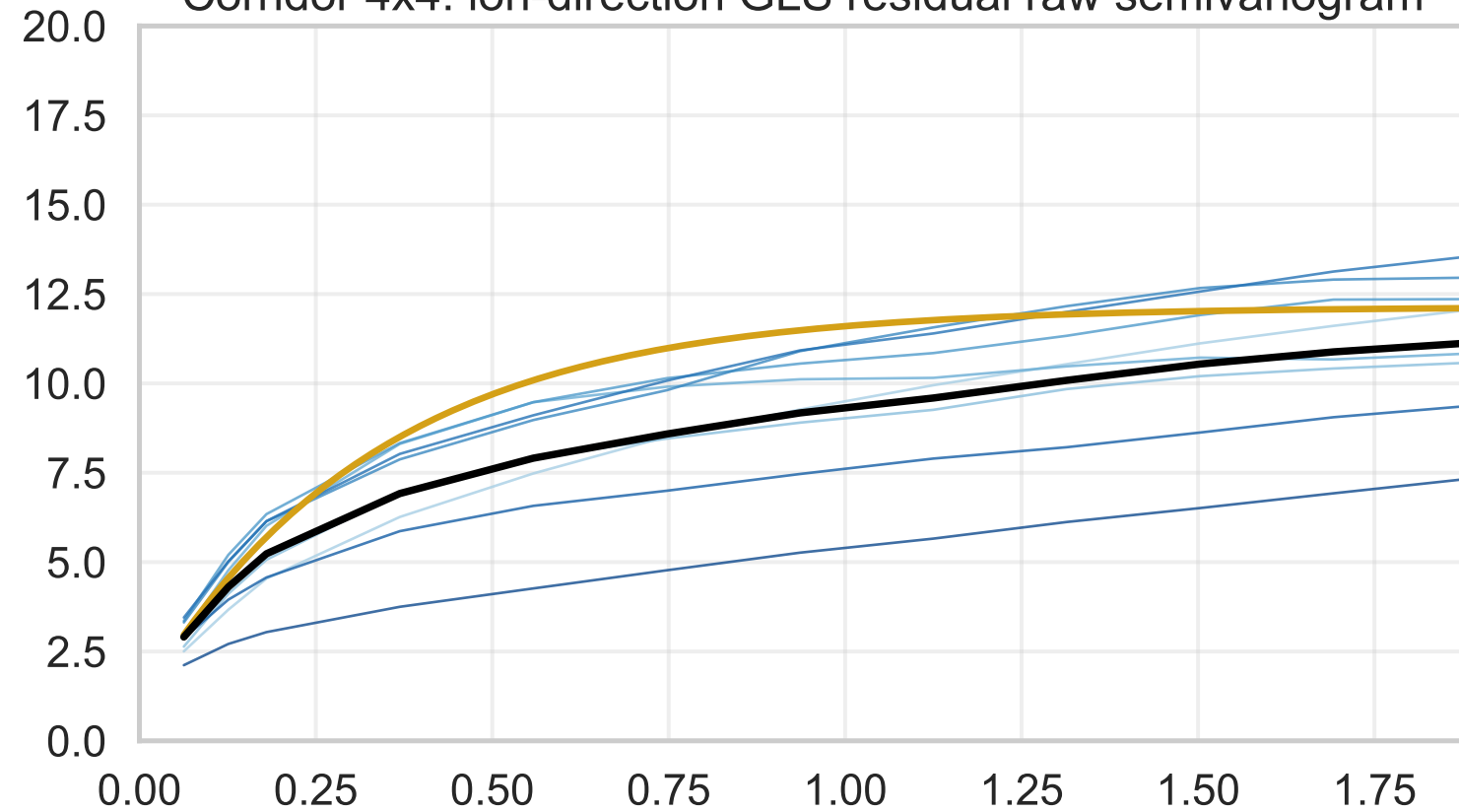
Corridor 4x4: lon-direction GLS residual raw semivariogram
