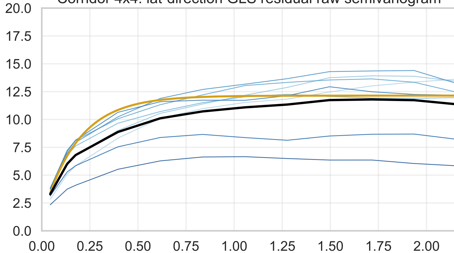
Corridor 4x4: lat-direction GLS residual raw semivariogram
