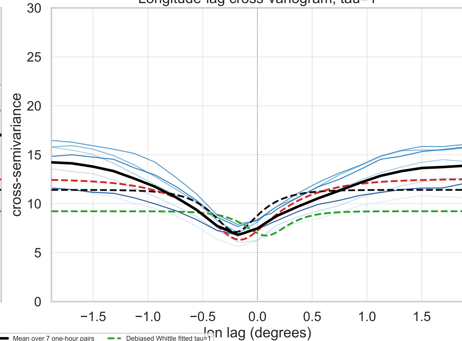
Longitude-lag cross-variogram, tau=1
