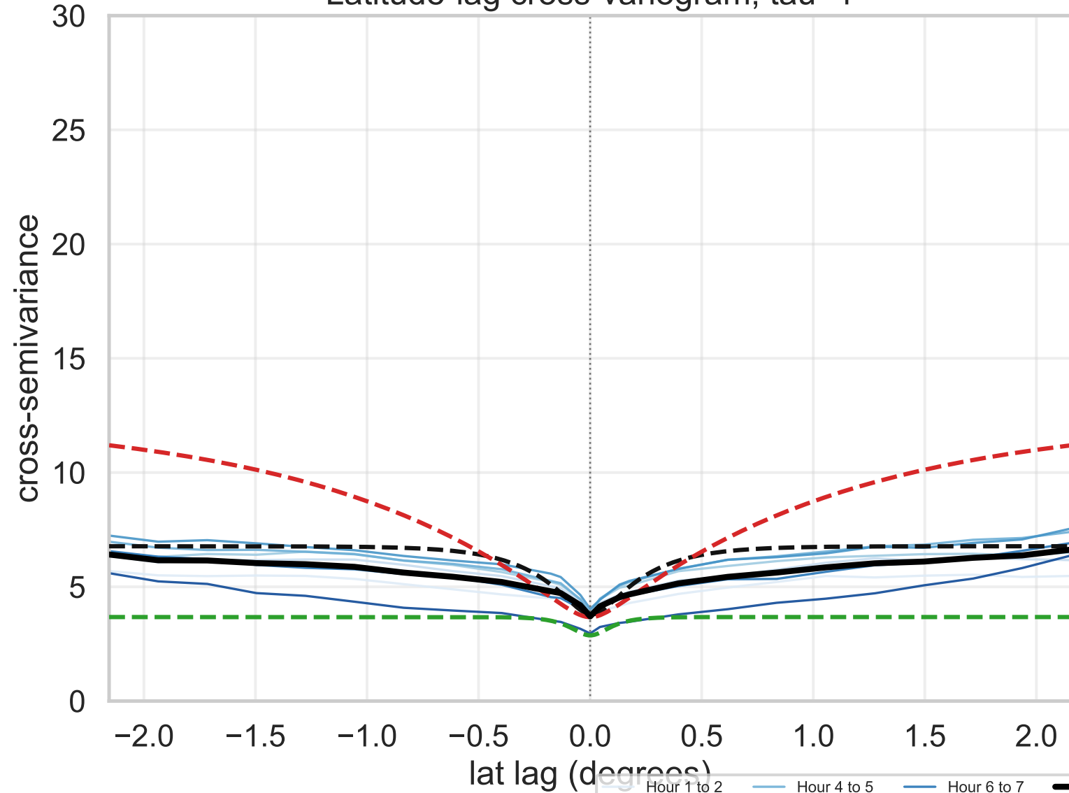
Latitude-lag cross-variogram, tau=1
