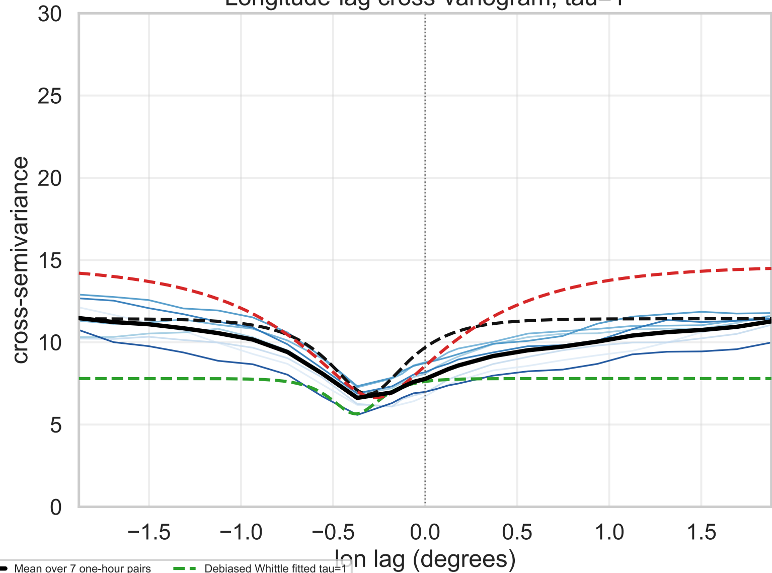
Longitude-lag cross-variogram, tau=1
