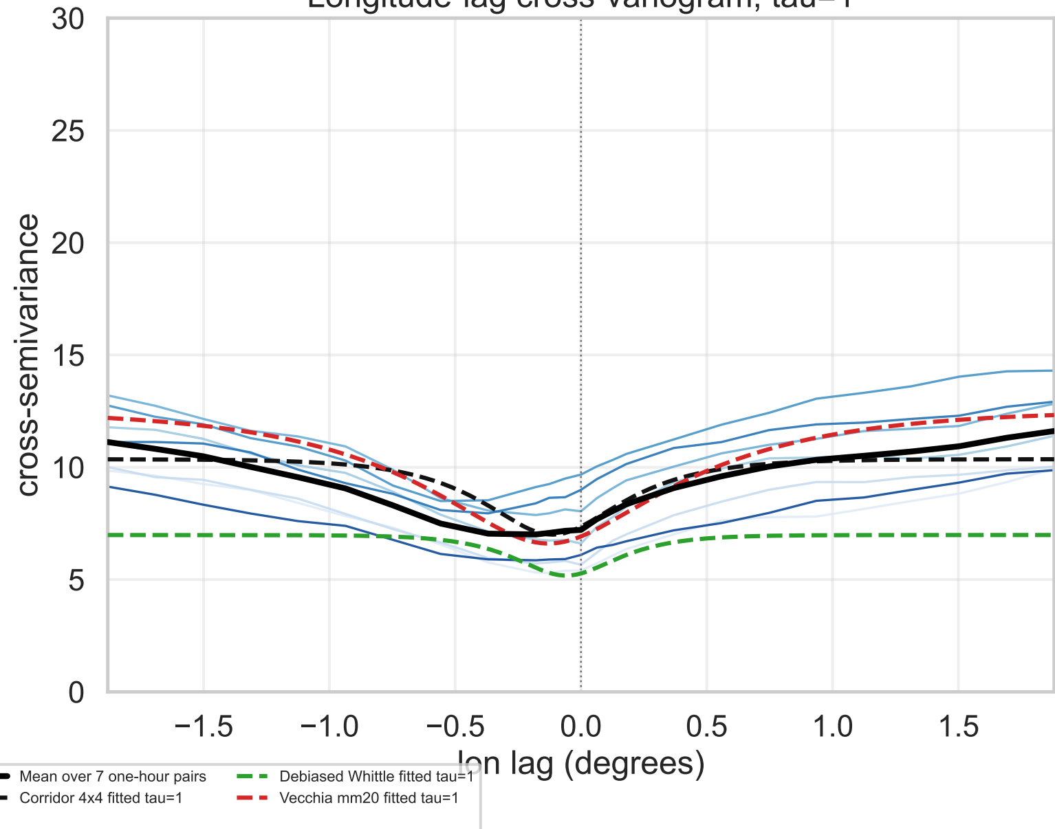
Longitude-lag cross-variogram, tau=1
