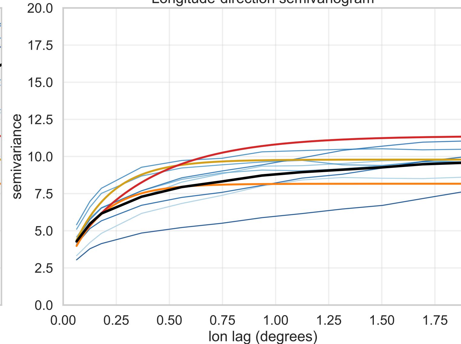
Longitude-direction semivariogram
