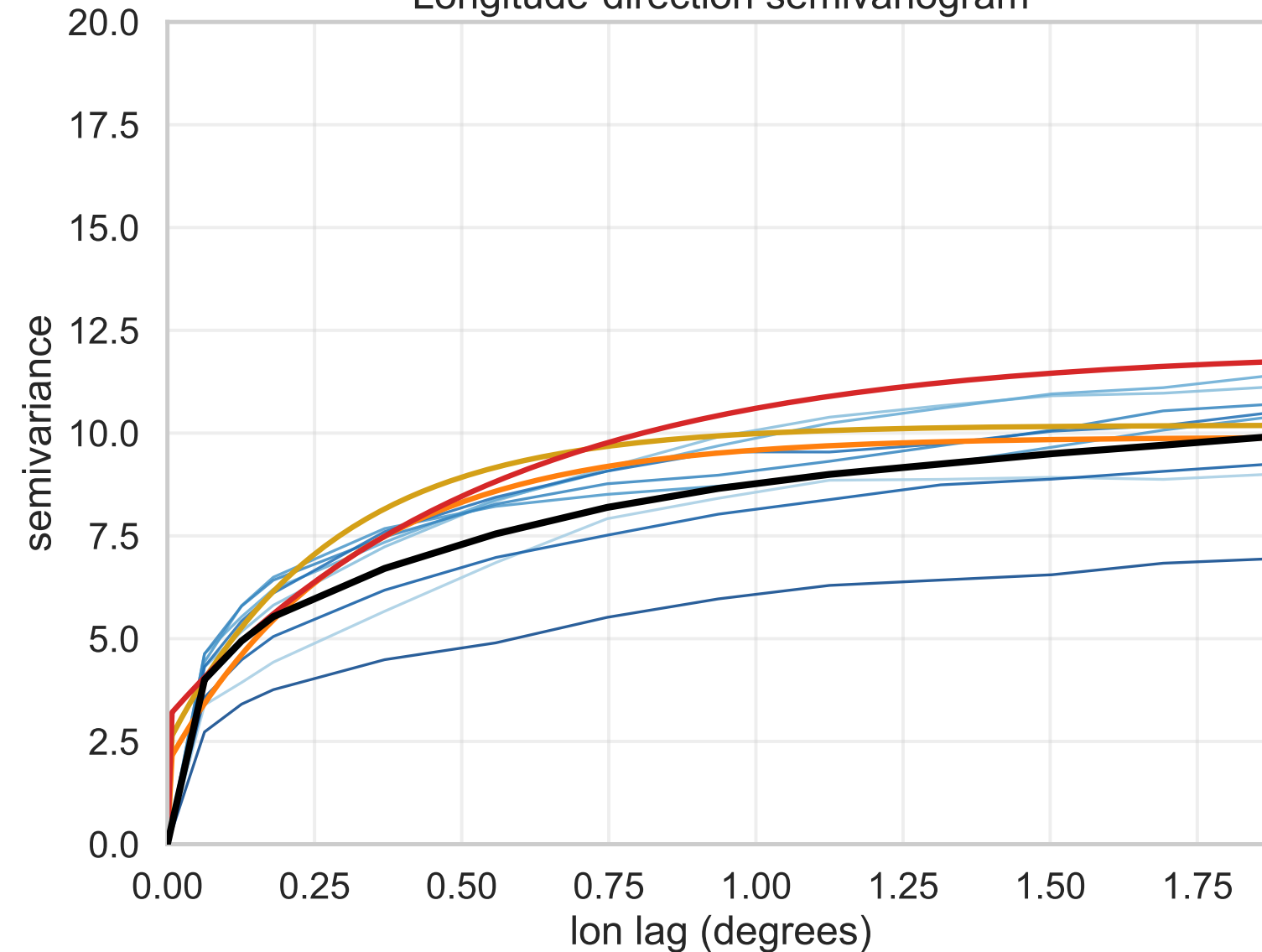
Longitude-direction semivariogram
