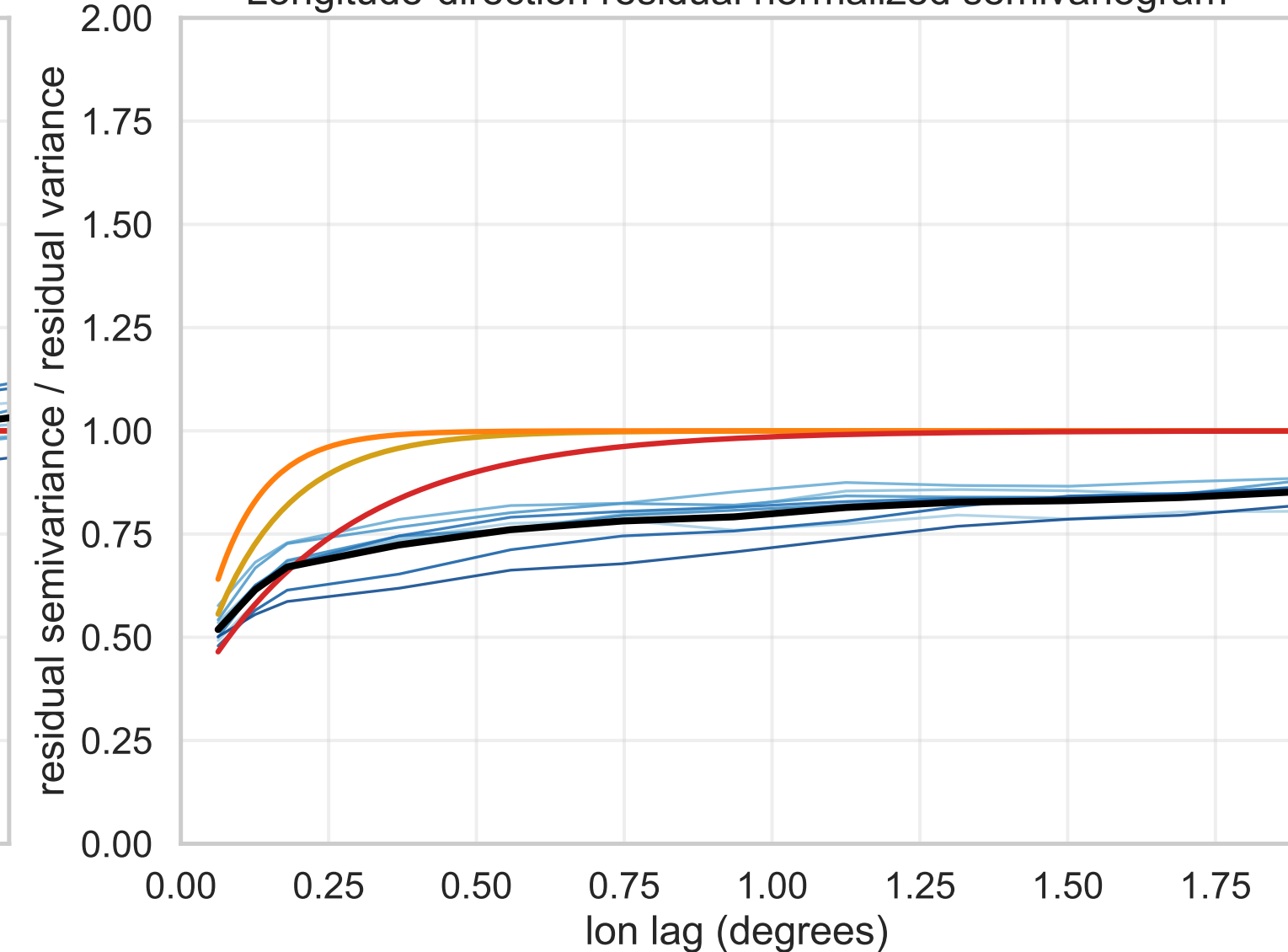
Longitude-direction residual normalized semivariogram
