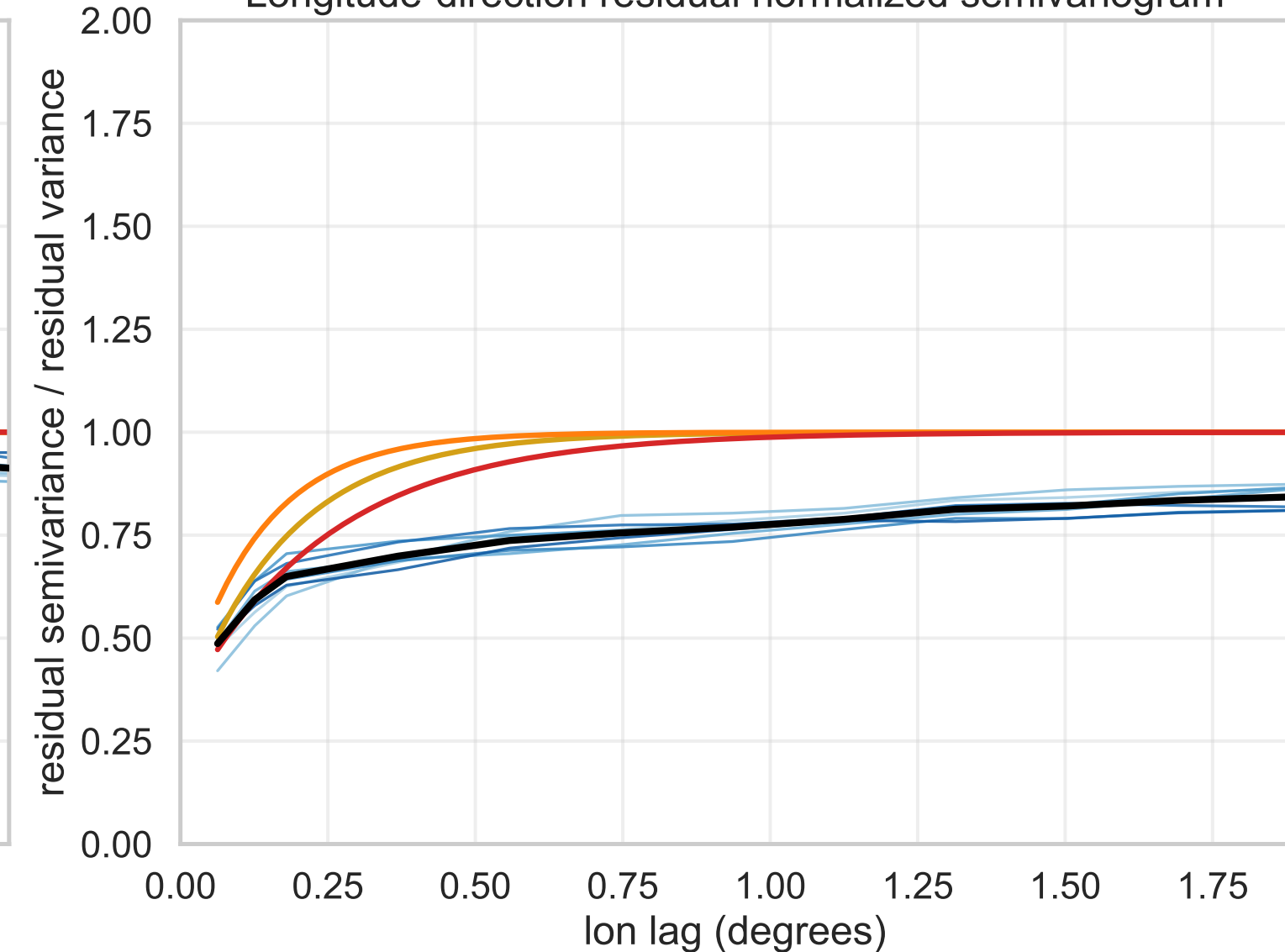
Longitude-direction residual normalized semivariogram
