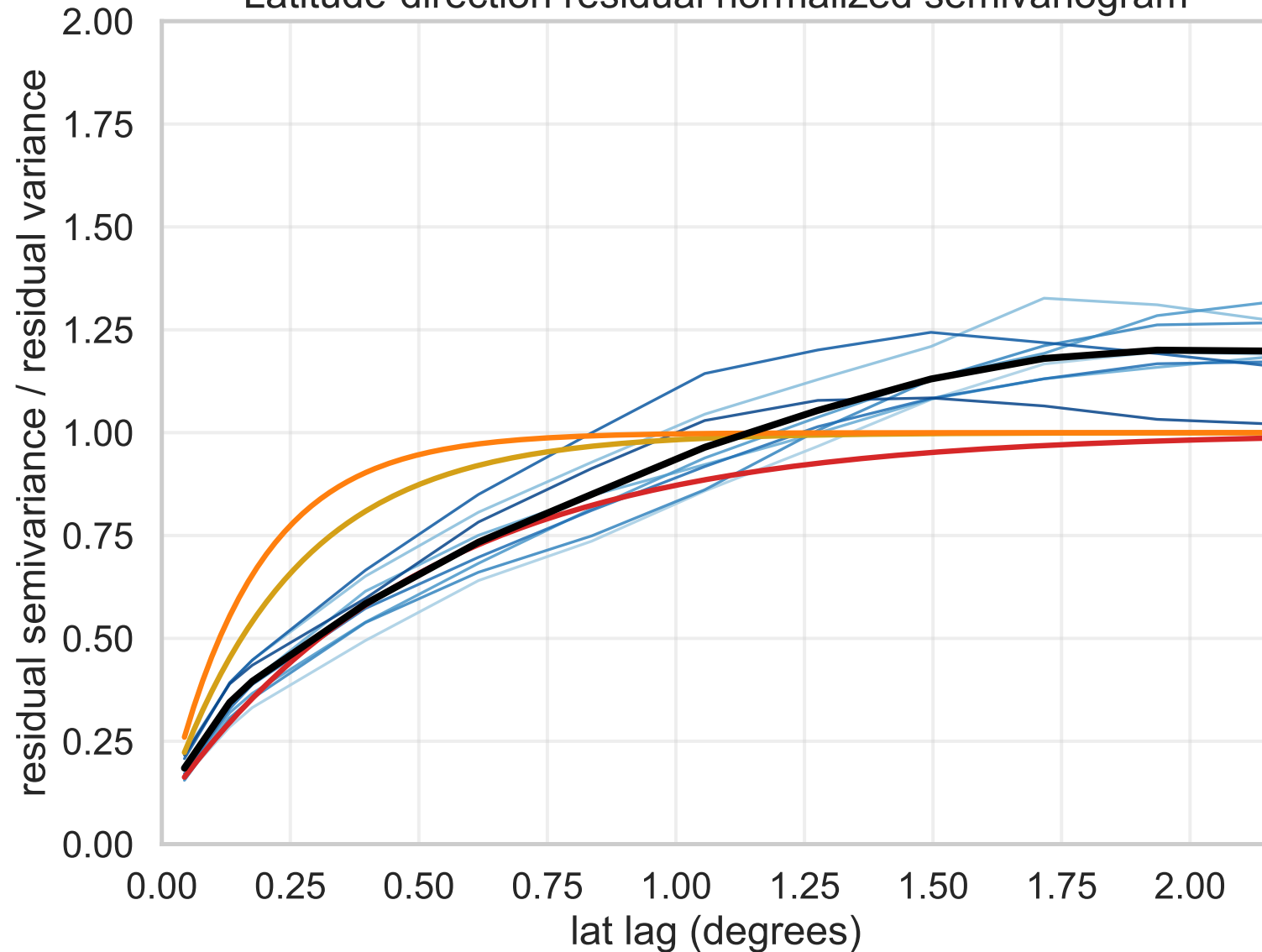
Latitude-direction residual normalized semivariogram
