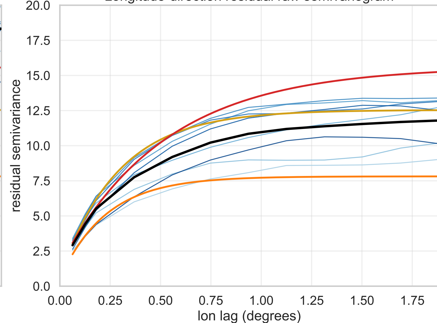
Longitude-direction residual raw semivariogram
