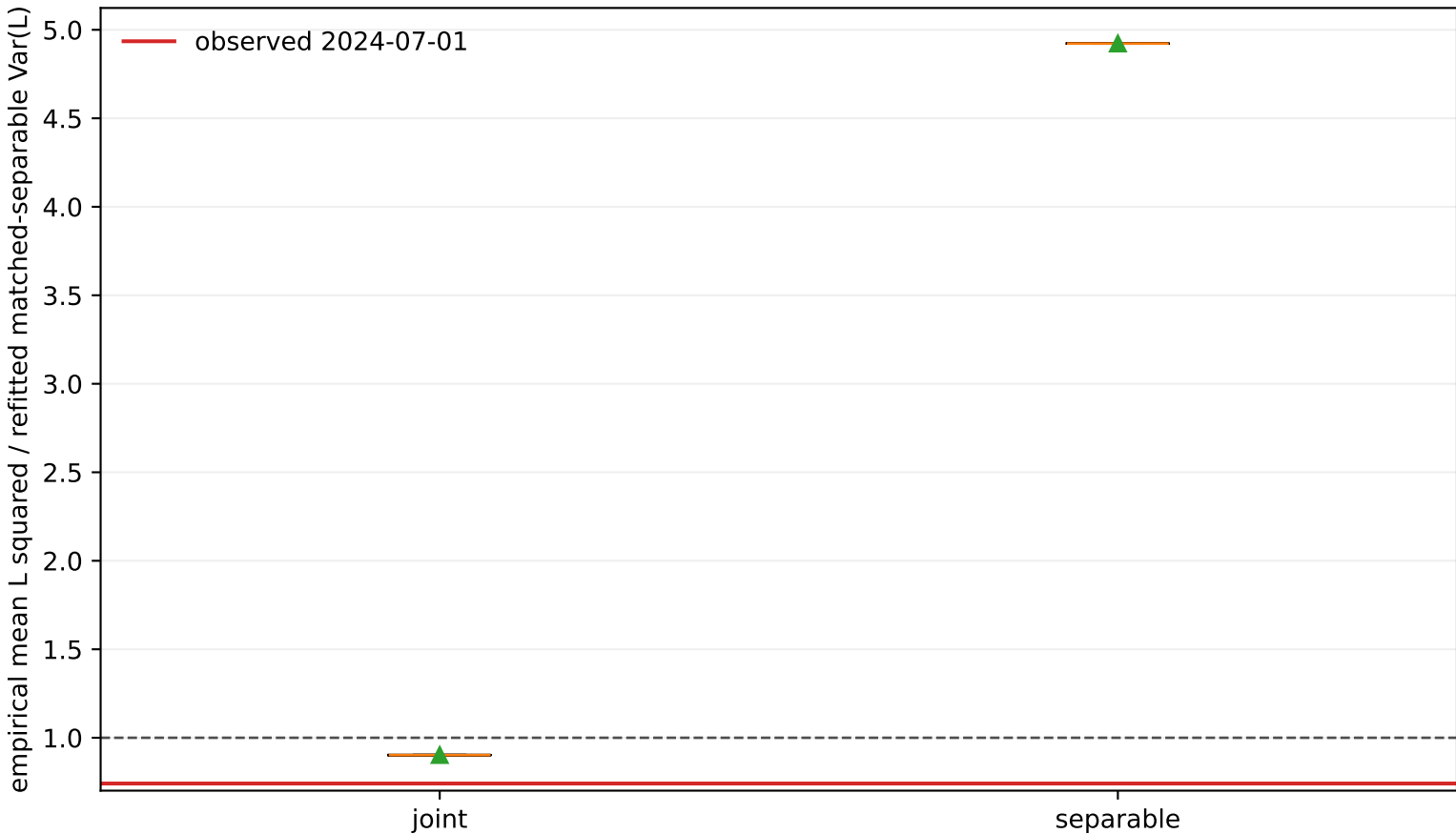
Frozen-contrast FFT/circulant full-pipeline bootstrap
