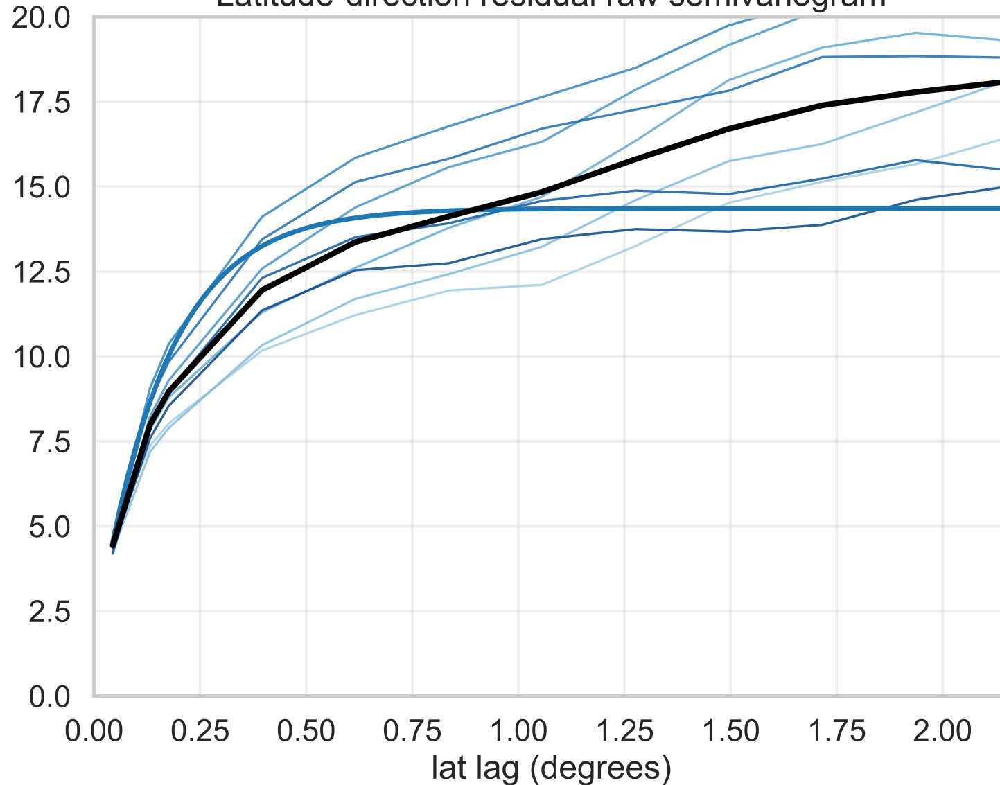
Latitude-direction residual raw semivariogram
