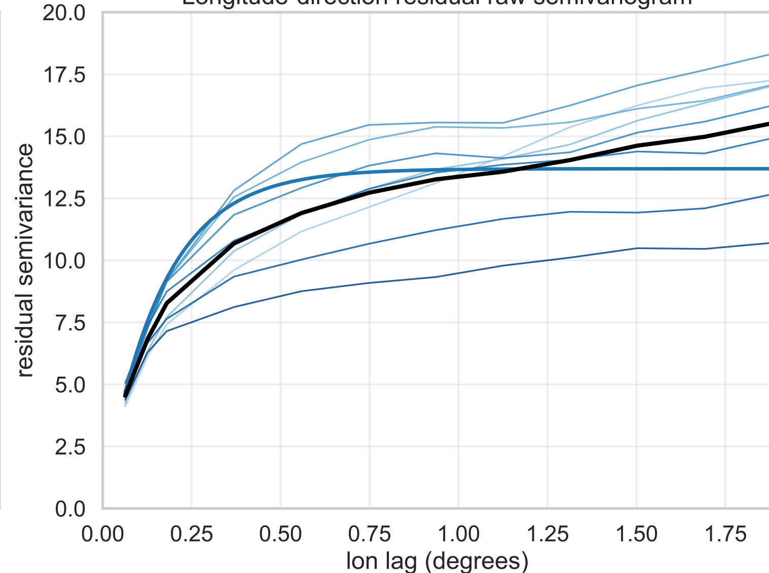
Longitude-direction residual raw semivariogram
