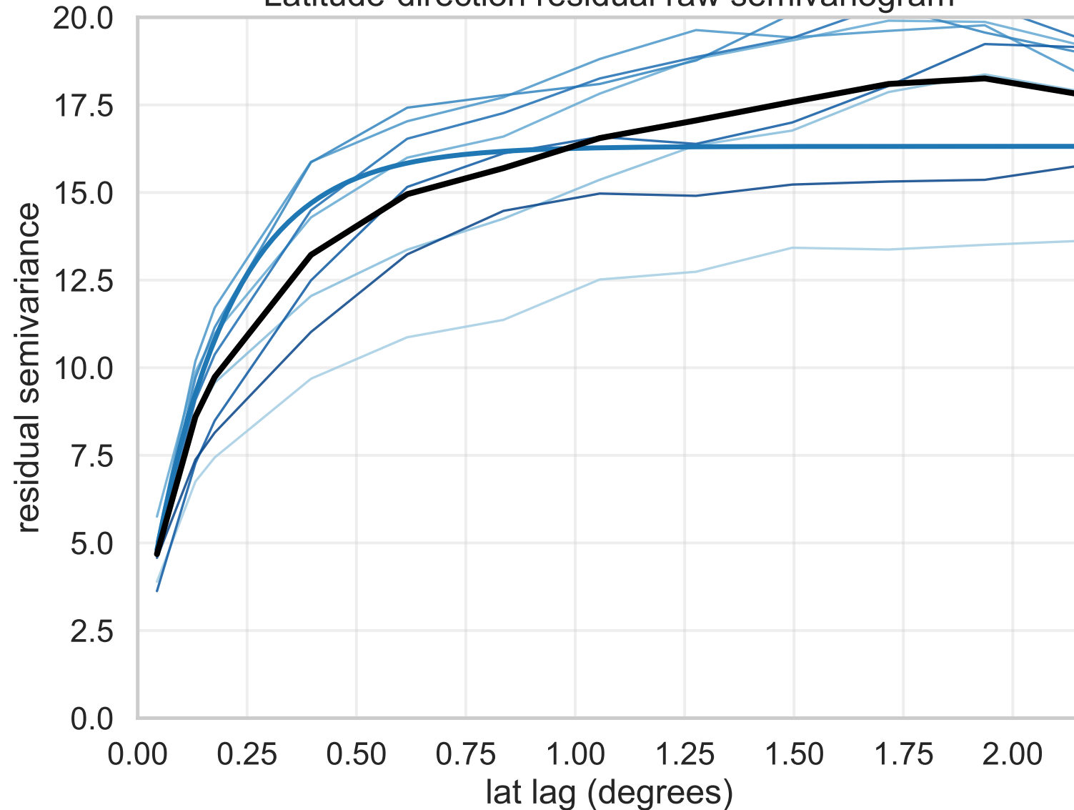
Latitude-direction residual raw semivariogram
