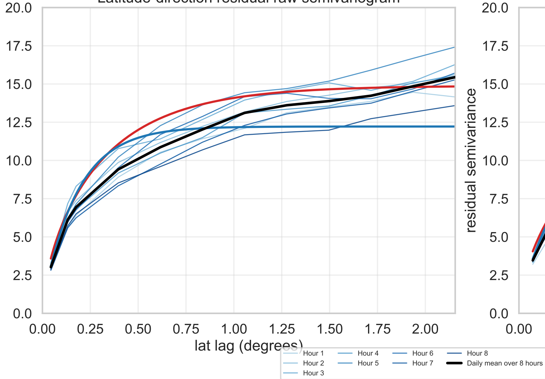
Latitude-direction residual raw semivariogram
