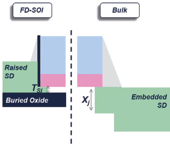
Figure 6: Comparison of DIBL effects in bulk CMOS versus FD-SOI technologies
