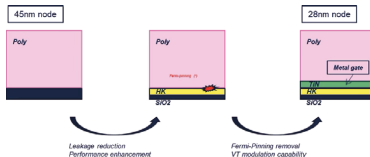
Figure 5: From SiON to high-K metal gate
