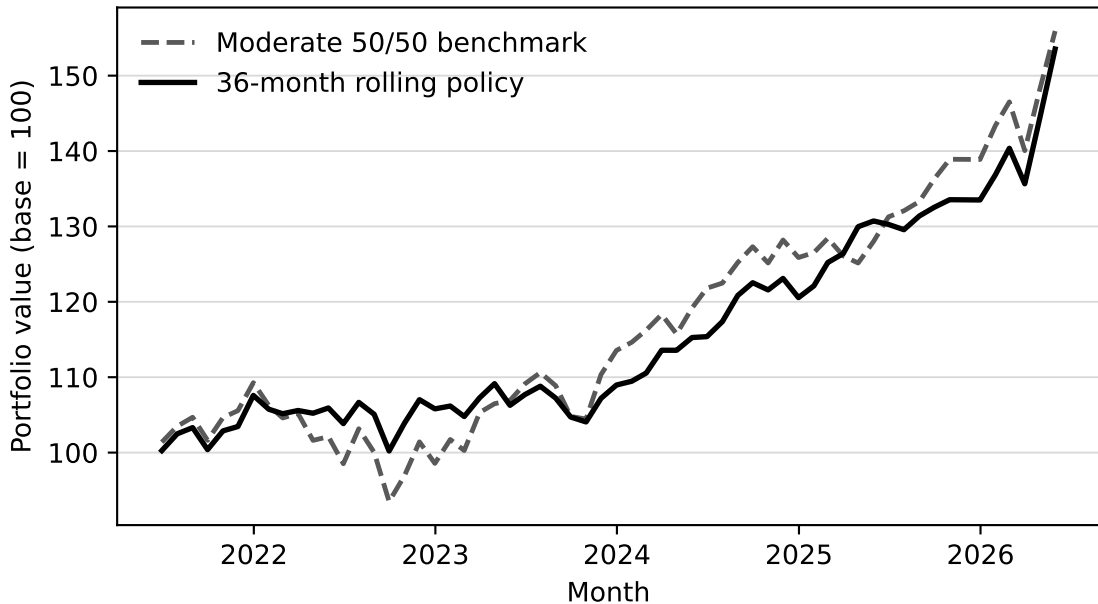
Moderate policy: normalized out-of-sample wealth
