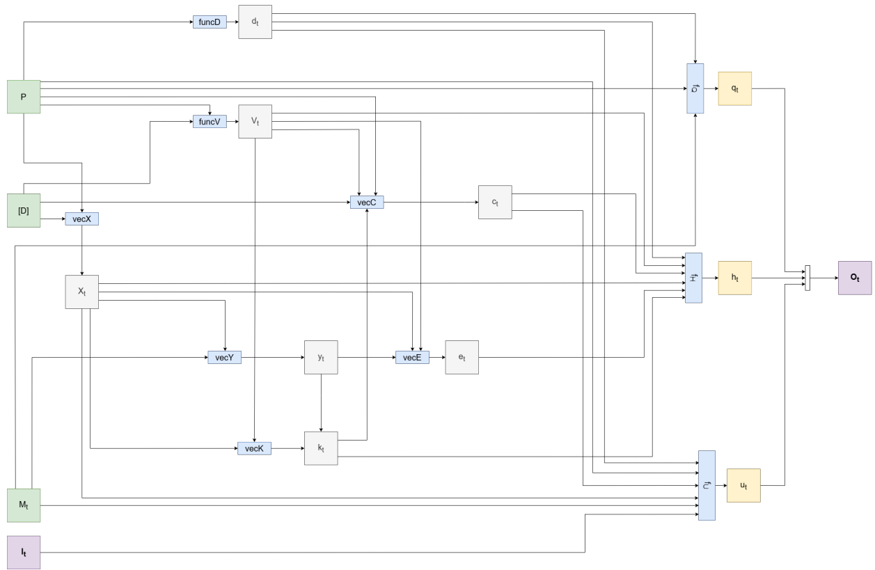
Figure 7: fEnc
