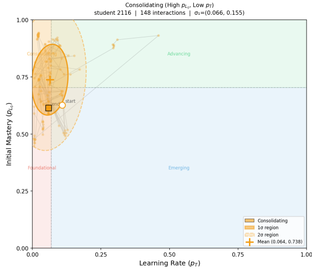
(b) Consolidating (high p_{L_0} , low p_T ): compact ellipse at high mastery and near-zero learning rate.
