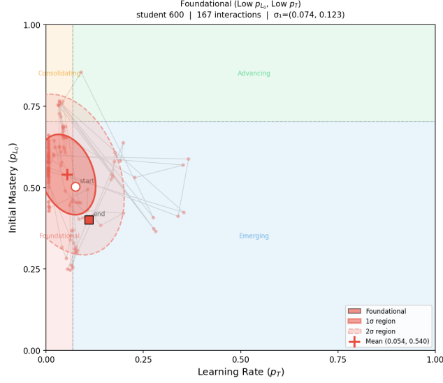
(a) Foundational (low p_{L_0} , low p_T ): compact ellipse at low mastery and low learning rate.
