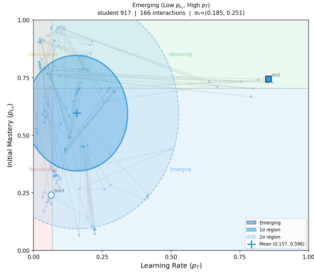
(c) Emerging (low p_{L_0} , high p_T ): most spatially extended ellipse, reflecting a heterogeneous profile across skills and interactions.
