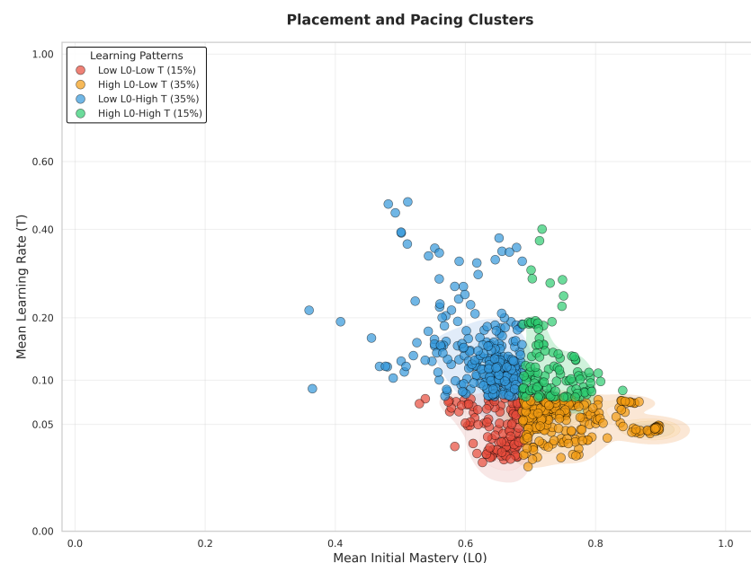
Figure 8. The figure shows the students clustered into four learning situations based on their historical learning parameters (computed as averages across all previous interactions).
