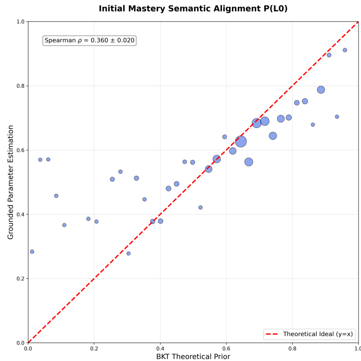
Figure 5. Semantic Alignment for Initial Mastery P_{L_0} . Plot showing weak monotonic relationship preservation (Spearman \rho = 0.360 , MAE = 0.168) between BKT theoretical priors and grounded parameters after neural transformation. Each bubble represents an aggregate of test interactions, with size encoding sample density. The substantial scatter indicates strong student-specific individualization, with the model prioritizing context-aware adaptation over strict adherence to population priors.
