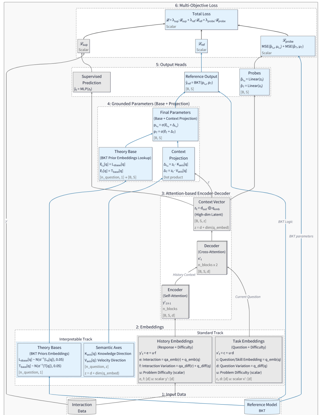
Figure 2. Functional layers of the gTransformer architecture. Gray denotes standard Transformer elements, blue denotes gTransformer-specific elements.
