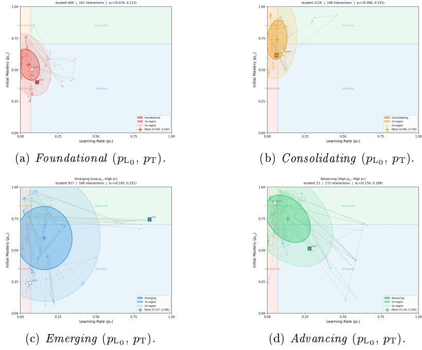
Fig. 3: Parameter orbit ellipses . Covariance ellipses ( 1\sigma and 2\sigma ) showing the grounded parameters distribution for the representative student of each learning situation. The centre marks the mean parameter position; ellipse shape encodes the extent and orientation of parameter variability across all interactions.
