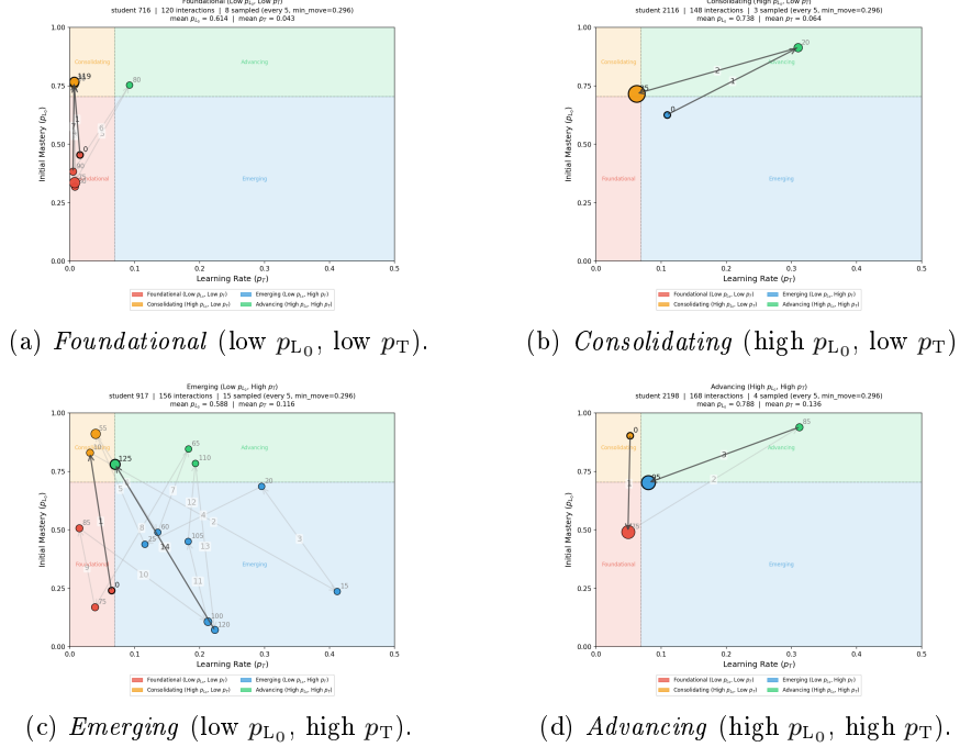
Fig. 4: Learning situation trajectories . Each plot traces the evolution of the grounded parameters pair for the representative student of one learning situation in the AS2009 dataset. Marker area encodes dwell time (interactions absorbed between two plotted points). The first and last arrows are rendered in a darker tone; all intermediate arrows are in light grey. The p_T axis is capped at 0.5. Coloured background regions delimit the four learning situations.
