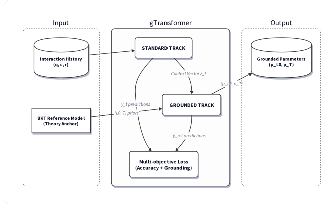
Fig. 1: The gTransformer architecture (adapted from [5]). The unified design integrates interaction history and theoretical priors through a dual-track engine to derive student-specific pedagogical signals ( p_{L_0}, p_T ).
